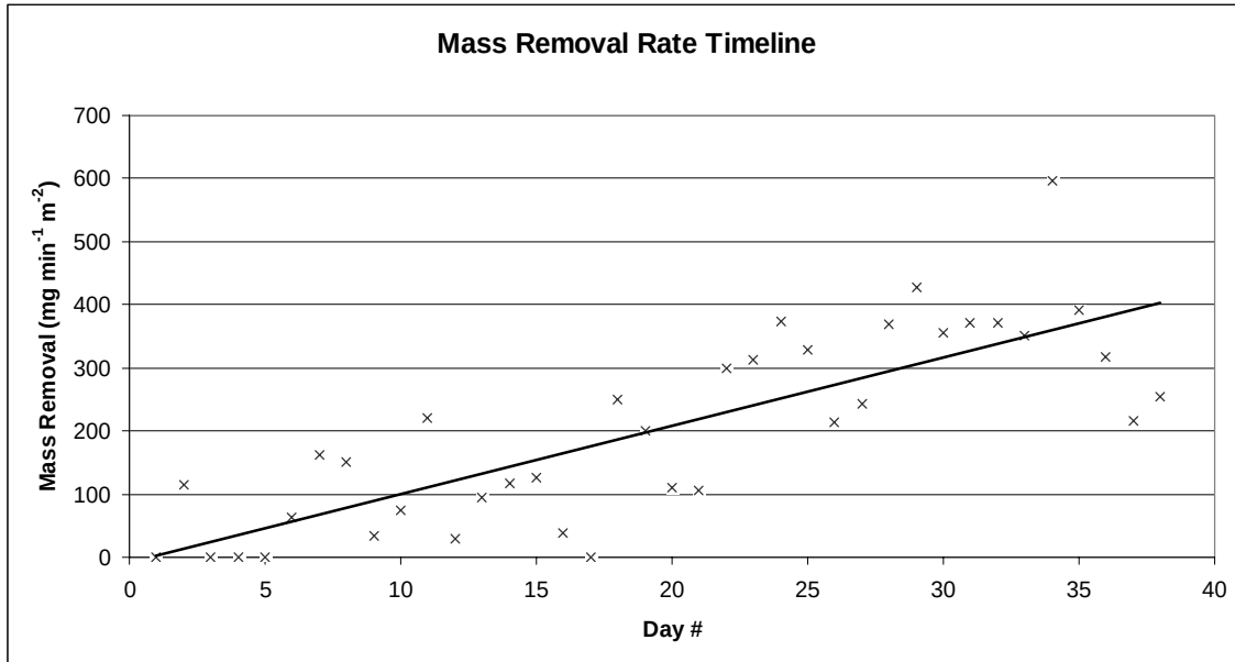
Figure 4.5: Mass Removal Rate Timeline. Cyclohexane removed based on membrane surface area. The trend line was added to depict the overall increase in performance over the course of the research.
