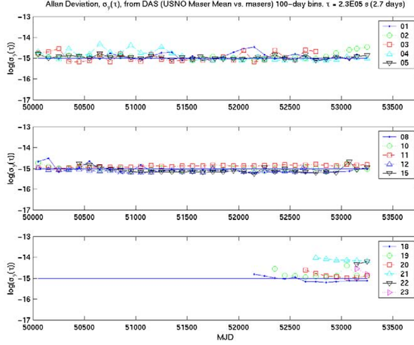
Figure 8. Allan deviation of individual USNO-DC masers for \tau = 64 hours (2.7 days), computed in 100-day batches.
