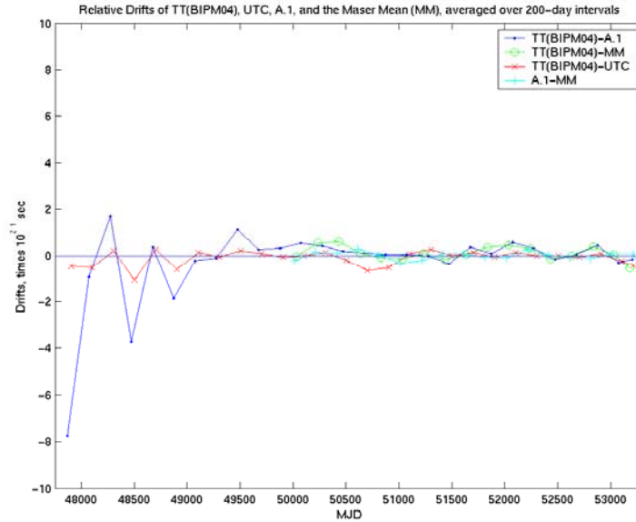
Figure 2. Frequency drifts between available timescale references. For display, the drifts have been multiplied by 10^{21} sec.
