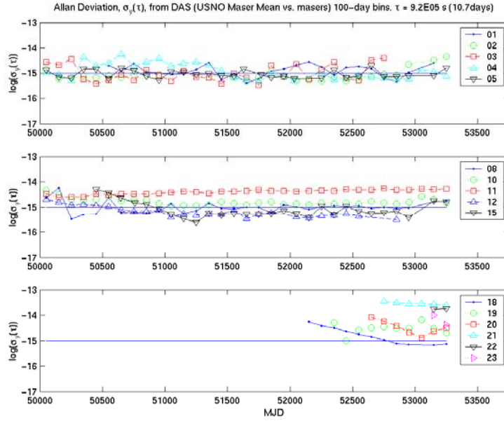
Figure 9. Allan deviation of individual USNO-DC masers for \tau = 256 hours (10.7 days), computed in 100-day batches.
