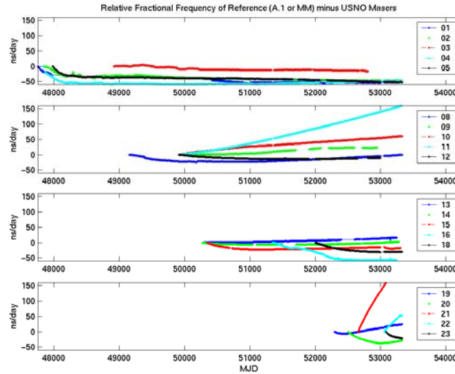
Figure 5. USNO maser frequencies. Masers are identified by their USNO designations. NAV 1 through NAV8 are referenced to A.1, and the others are referenced to the USNO Maser Mean. The maser NAV15 failed on MJD 53307 due to a problem within its physics package.
