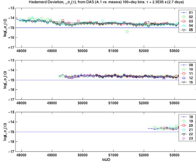
Figure 10. Hadamard deviation of individual USNO-DC masers for \tau = 64 hours (2.7 days), computed in 100-day batches.
