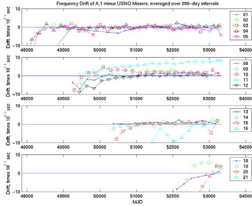
Figure 7. Frequency drifts of USNO masers located in Washington, DC (USNO-DC), computed by differencing frequencies at endpoints of 200-day intervals. Since MJD 49000, the frequency drifts between the A.1, UTC, and TT (BIPM03) have been less than 10^{-21} /sec. The maser NAV21 has drifts of order 4\text{--}5 \times 10^{-20} /sec.
