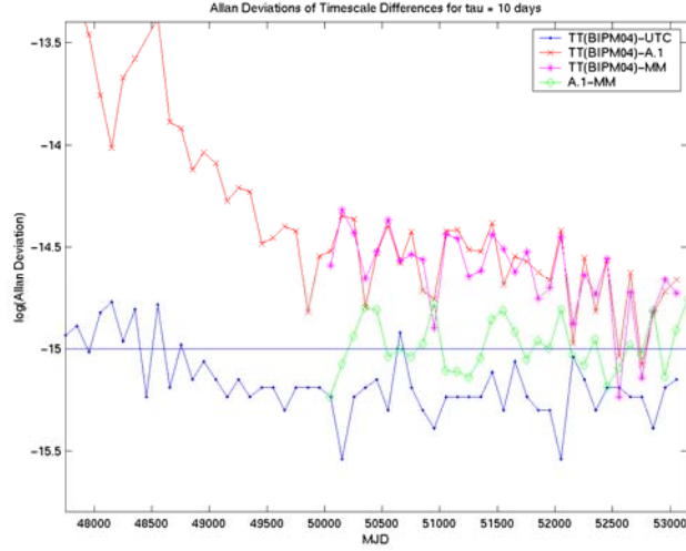
Figure 3. Allan deviation of differences between external and internal timescales, for tau of 10 days. The greater stability of the more recent data is due to several improvements in timekeeping. The Hadamard deviations are numerically similar to the Allan deviations for such short averaging times.
