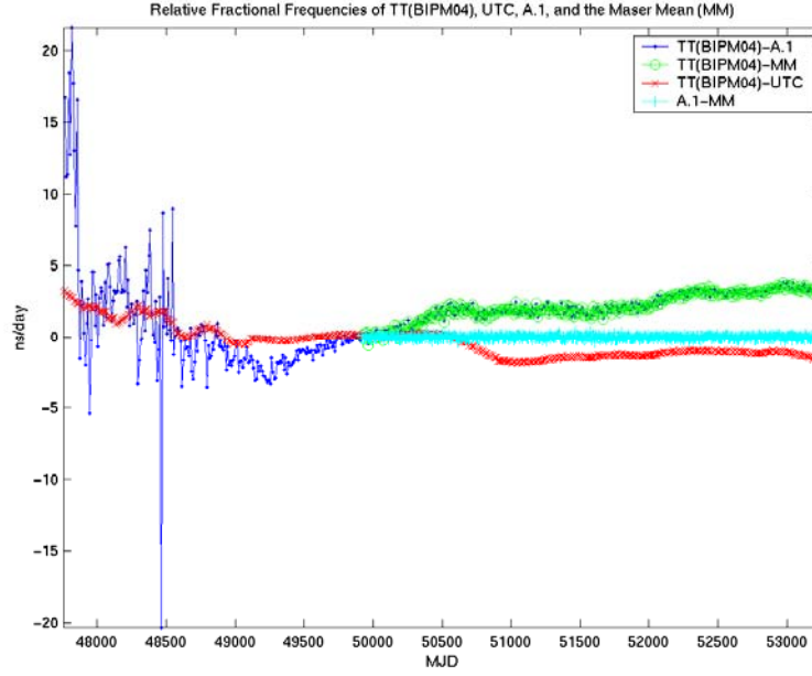
Figure 1. Fractional frequency differences between references used in this work. In all cases, the differences are less than the difference between individual masers and any one reference. The large variations before MJD 49000 (January 1993) reflect the significantly smaller number and higher instability of the existing cesium clocks (not shown), as well as the higher noise of pre-GPS time transfer.
