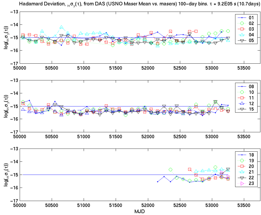
Figure 11. Hadamard deviation of individual USNO-DC masers for \tau = 256 hours (10.7 days), computed in 100-day batches.
