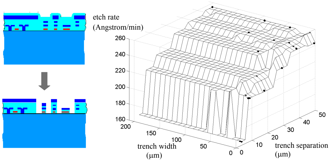
FIGURE 11. Etch lag of RIE oxide on different test trench patterns with an 170 min etch and O 2 flow at 5 sccm. Note the scale is much larger than in the previous figure.
