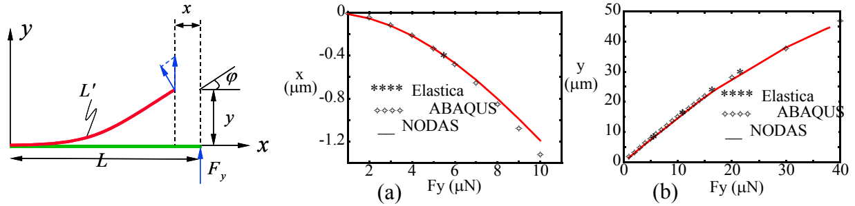
FIGURE 35. Static analysis of a cantilever beam ( L=100 \mu\text{m} , w=2 \mu\text{m} , t=2 \mu\text{m} , E=165 \text{ GPa} ) under a force in y -direction (a) displacement in x ; (b) displacement in y .
