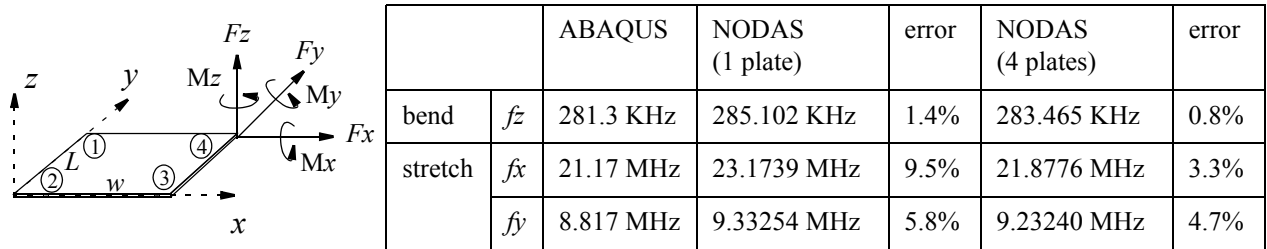
FIGURE 36. (a) 3-D elastic plate (b) comparison of NODAS and ABAQUS simulation results ( L=100 \mu\text{m} , w=100 \mu\text{m} , t=2 \mu\text{m} , E=165 \text{ GPa} ).
