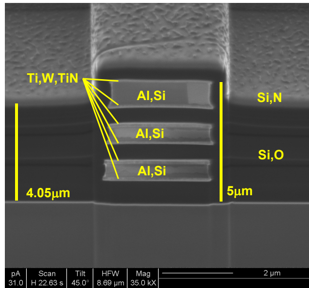
FIGURE 4. FIB cross-section from the first alpha run in the AMS 0.6 \mu m CMOS, before micromachining steps.
