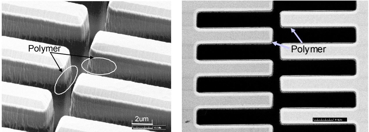
FIGURE 13. SEM images showing (a) sidewall polymerization and (b) structural bloat.
