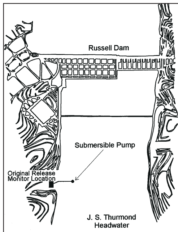
Figure 7. Richard B. Russell original downstream monitor
