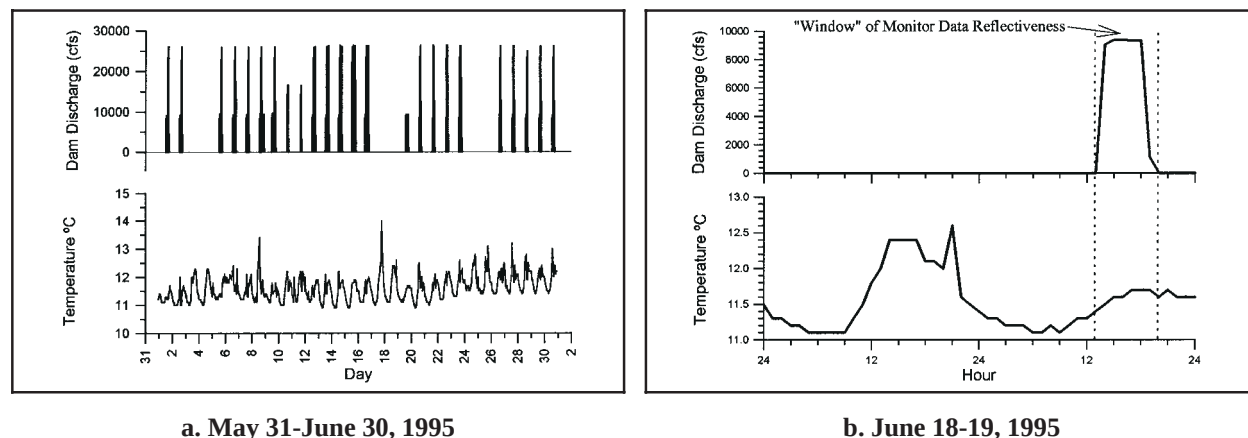
Figure 6. Hartwell Dam operation and release temperatures
