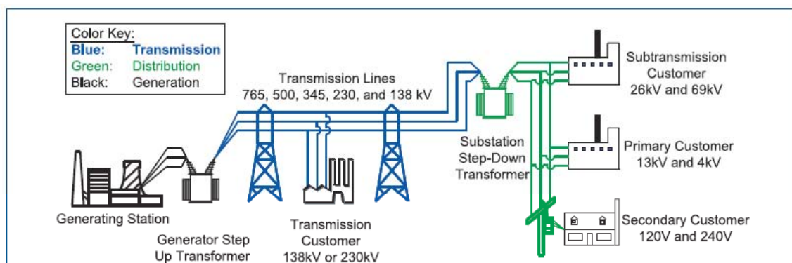
Figure 8 Basic Structure of the Electric System, https://reports.energy.gov/B-F-Web-Part1.pdf
