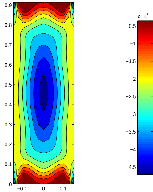
Figure 83. Bottom Surface S22 Stress Contour
