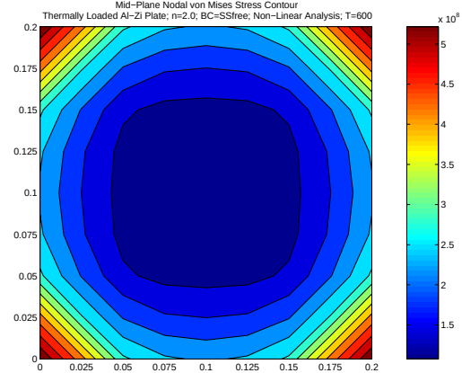
Figure 43. Plate-Thermally Induced Stress for n=2.0 (Non-Linear)
