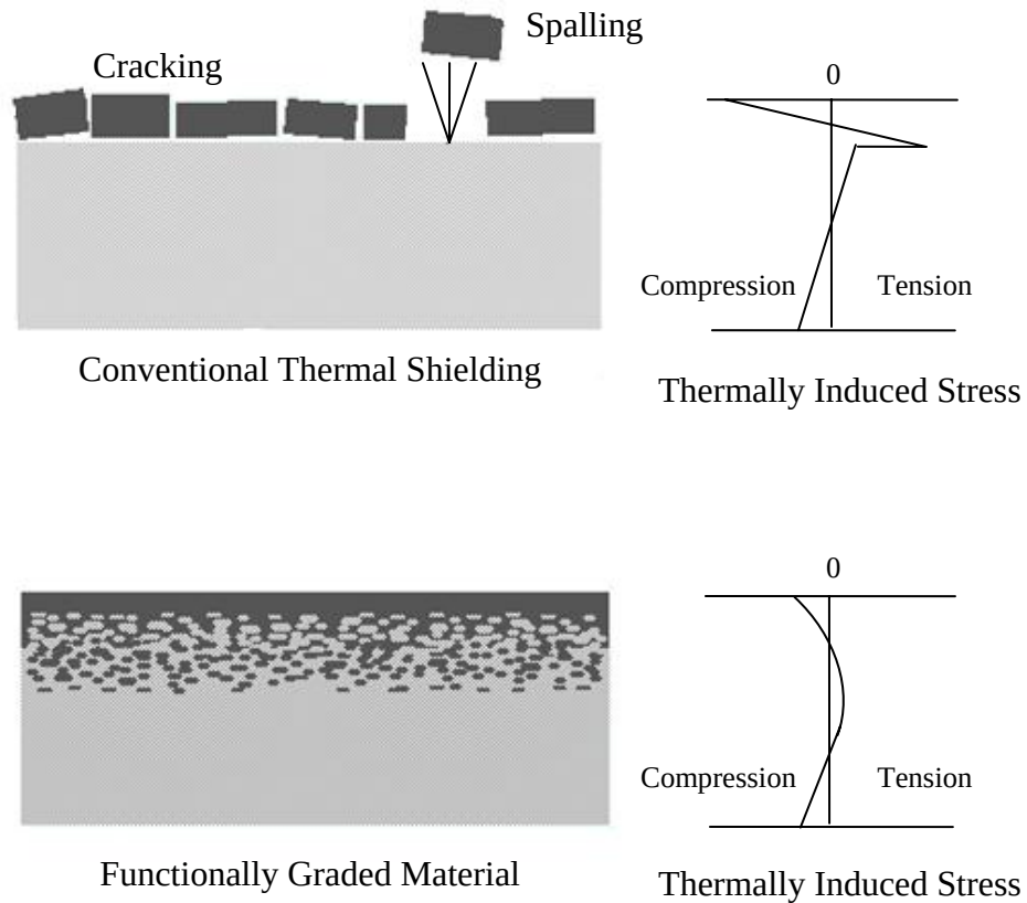
Figure 1. Thermal Protection
