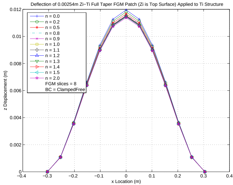
Figure 140. Exhaust Wash Deflection with 0.1" Zi-Ti FGM Full Taper Patch
