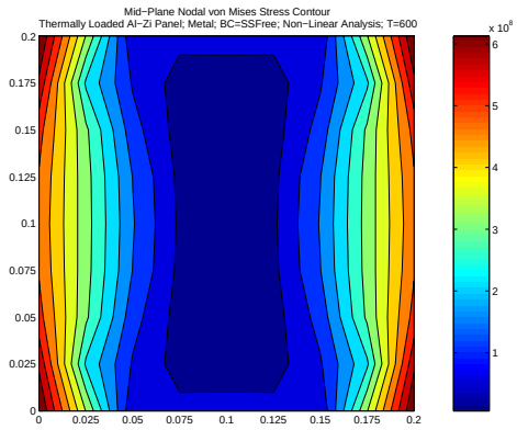
Figure 80. Panel-Thermally Induced Stress for n=Metal (Non-Linear)
