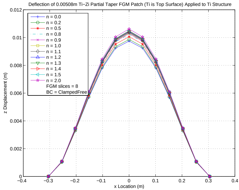
Figure 114. Exhaust Wash Deflection with 0.2" Ti-Zi FGM Partial Taper Patch
