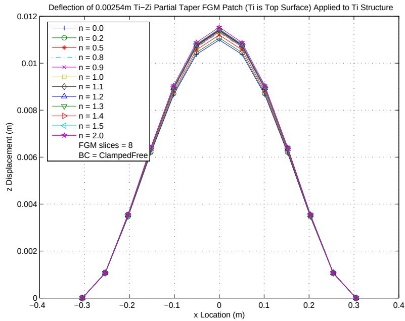
Figure 113. Exhaust Wash Deflection with 0.1" Ti-Zi FGM Partial Taper Patch
