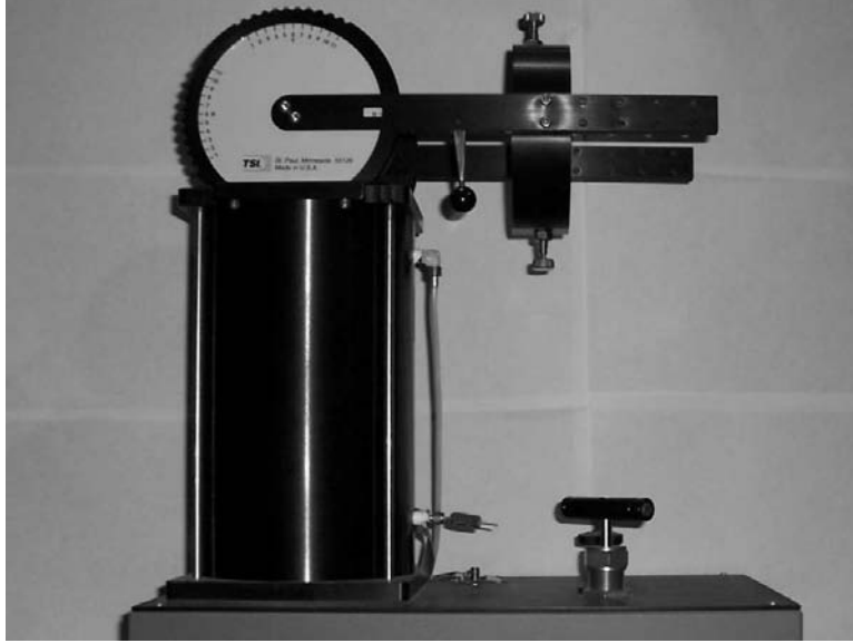
Figure 3.19: Apparatus used to calibrate a hot film anemometer.
