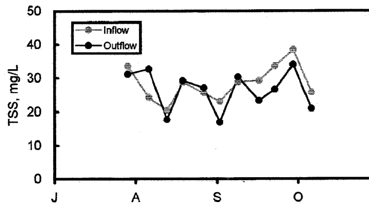
b. Total suspended sediment (TSS)
