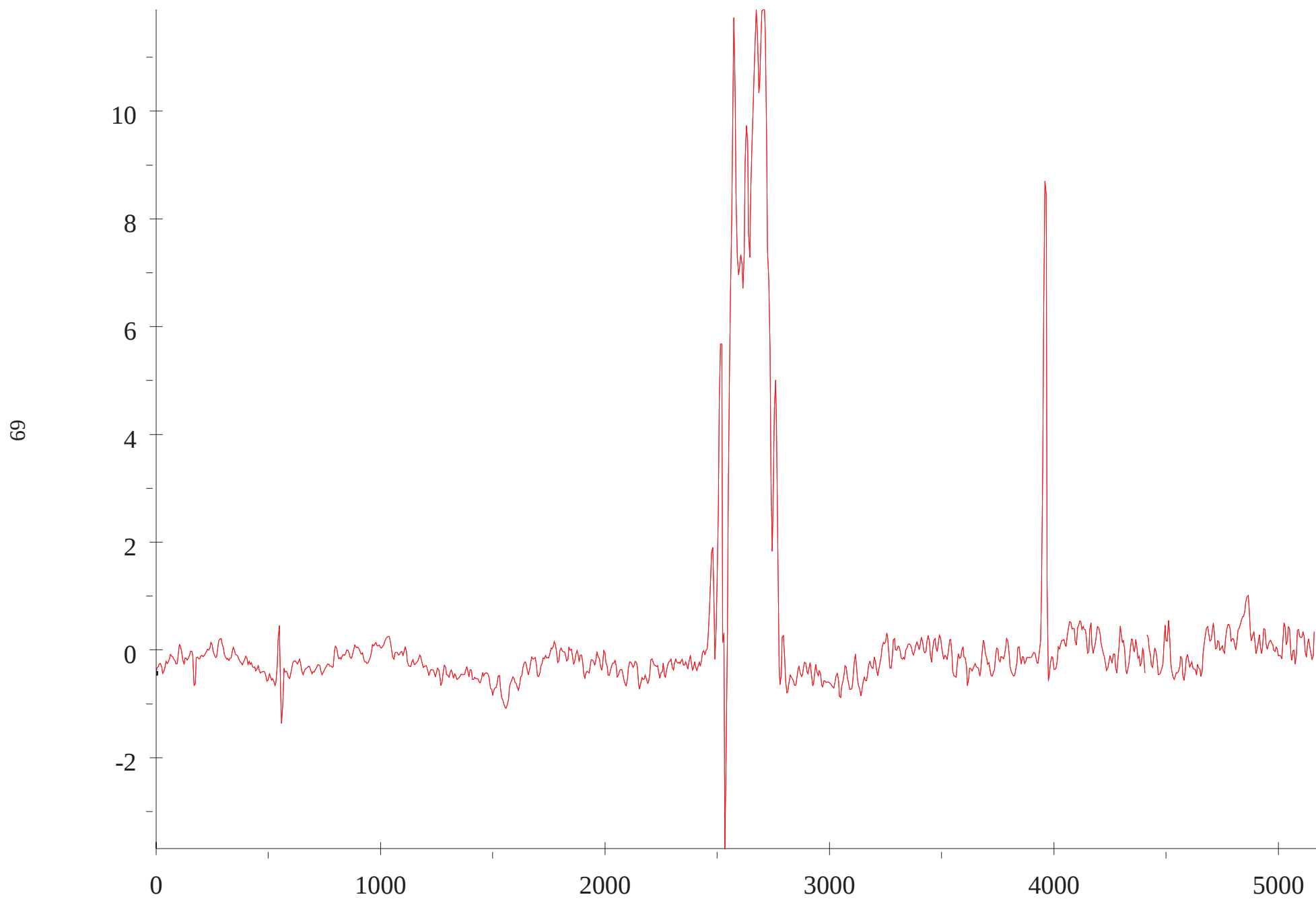
Figure 50. Difference Cross-section of the First LIDAR Delivery and Corrected IFSAR
