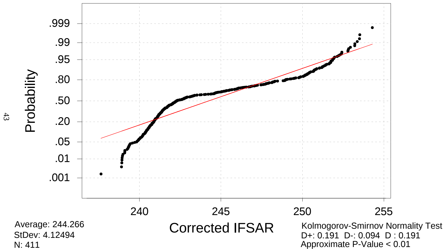
Figure 29. Normal Probability Plot for the LIDAR DEM Data
