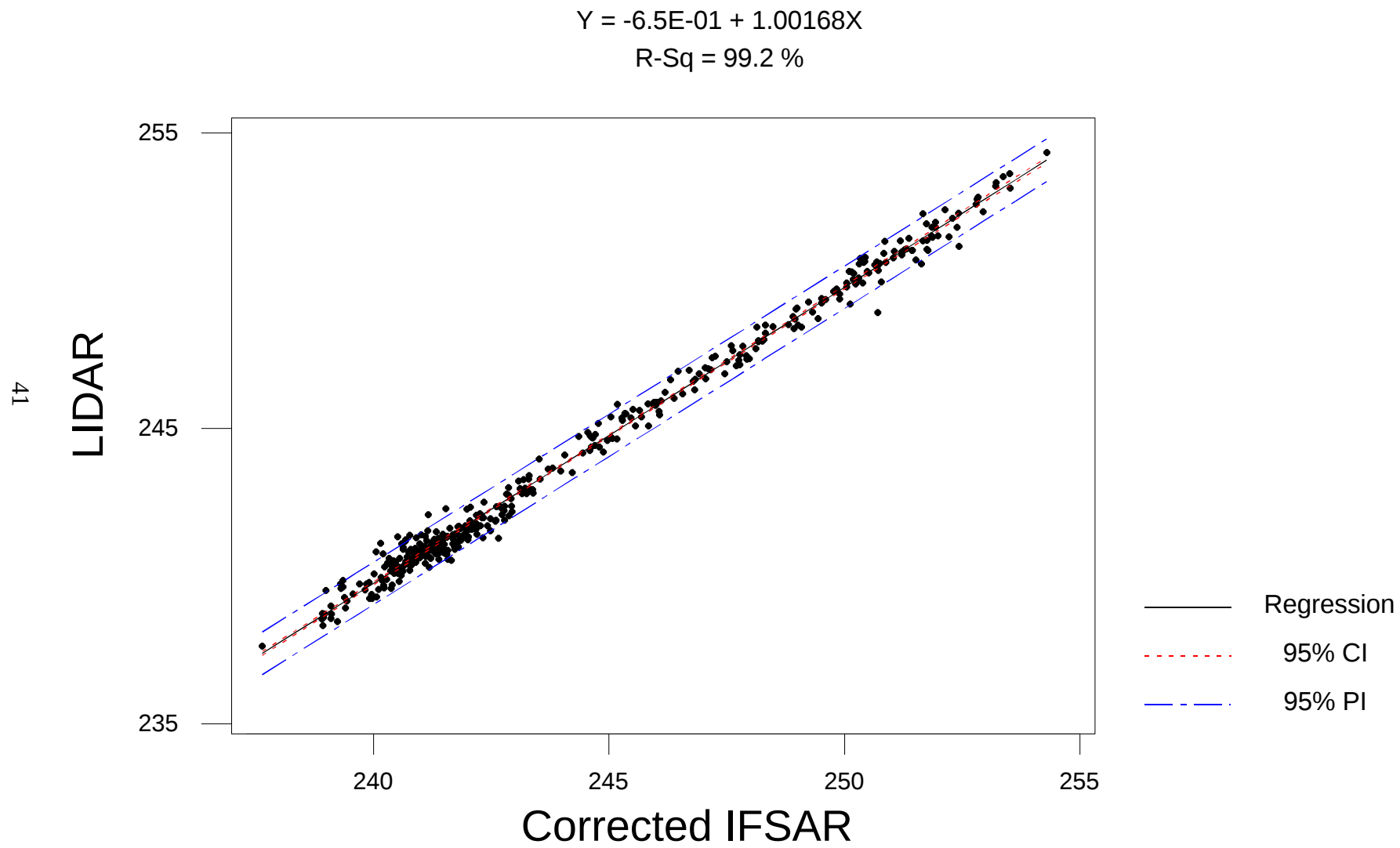
Figure 27. Regression Plot
