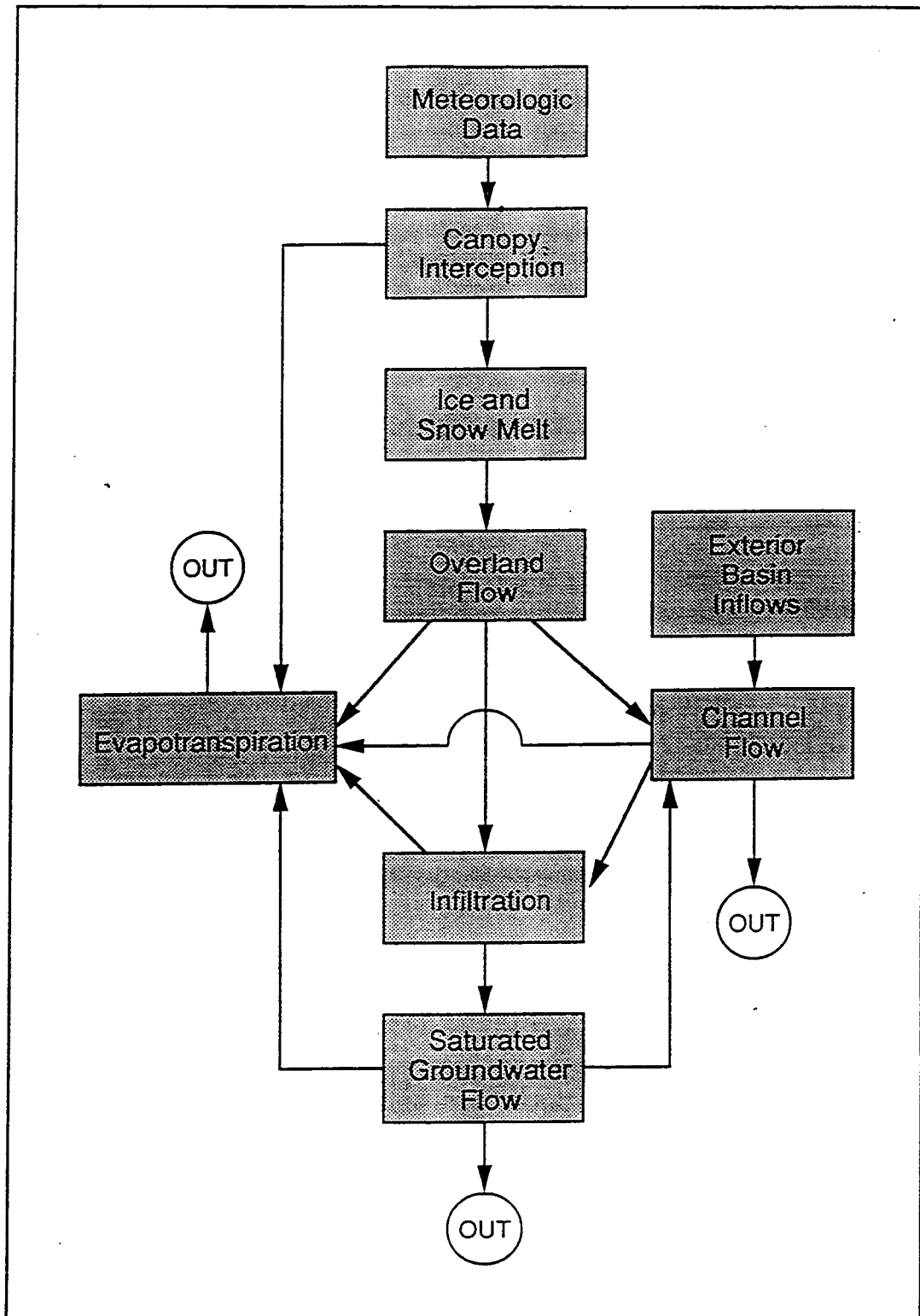
Figure 1. Schematic processes
