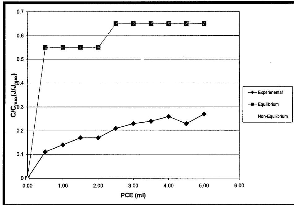
Figure 3.21. 20/30 curve comparison
