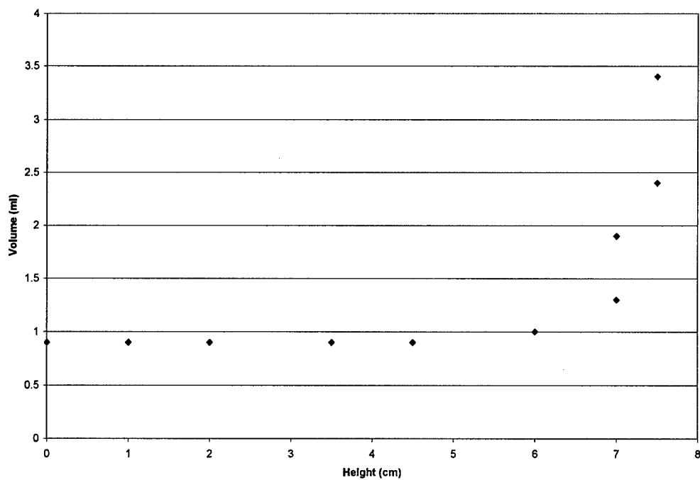
Figure A.9. 75% OTS treated water entry pressure (air saturated)
