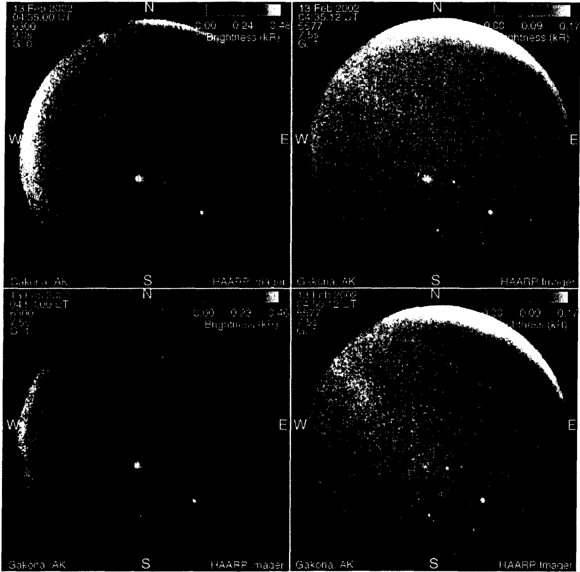
Fig. 3. Heater-induced red- and green-line emissions during the long pulse before (top) and after (bottom) f_oF_2 has dropped below f_0 . Bold circles mark the heated spot at MZ. Bright dots outside the circles are stars. The color bars show the brightness from 0 to 0.48 kR and from 0 to 0.17 kR for the red- and green-line emissions, respectively.
