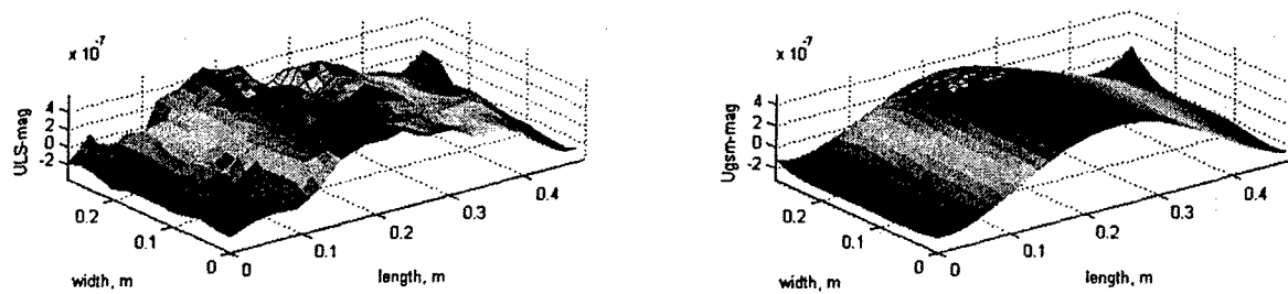
Figure 33 The ULS and U_{GSM} of Comp-CC-ED using the first 3 curvature mode shapes from the PVDF sensor system
