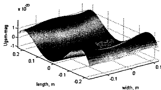
Figure 25 The ULS and U_{GSM} of Comp-CC-ED using the first 3 longitudinal bending mode shapes from the SLV system
