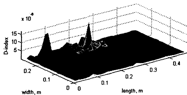
Figure 34 DI distribution of Comp-CC-ED using ULS from the first 3 curvature mode shapes from the PVDF sensor system
