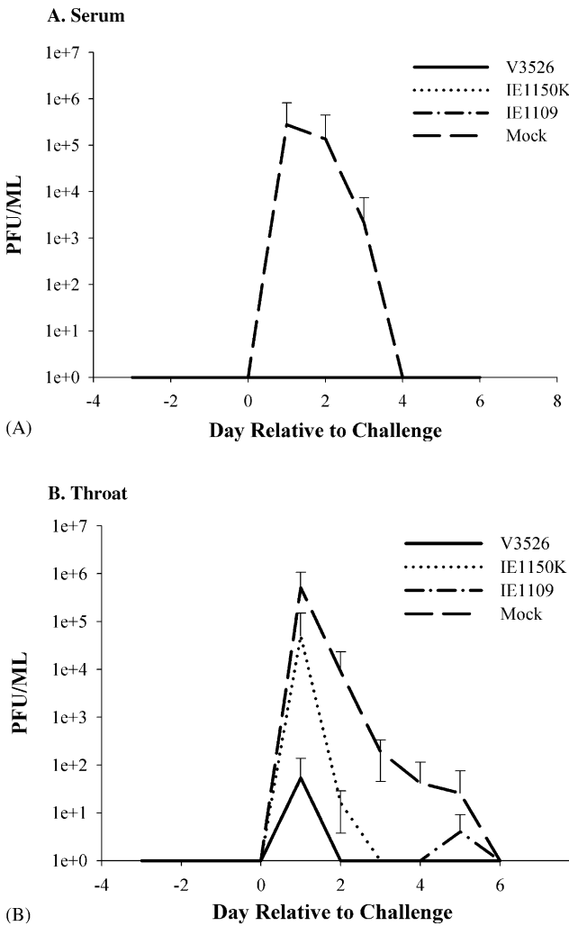
Fig. 3. Virus isolation from the throat and serum after aerosol exposure of macaques to VEEV-IE. Blood samples (A) and throat swabs (B) taken daily from days –3 to +6 were examined for the presence of virus by plaque assay in Vero cells. Graphs show the mean virus concentration in PFU/ml \pm S.D. for V3526-, IE1150K-, IE1109-, or mock-vaccinated macaques beginning on day –3 through day +6 relative to challenge.
