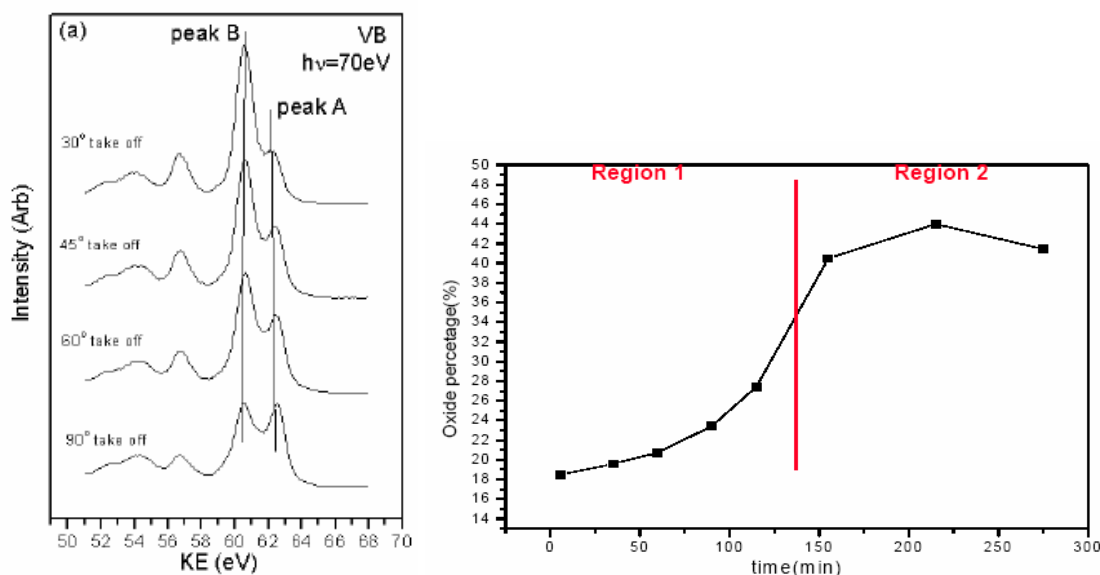
Figure 5. Left - Valance band at different incidence angles after activation. Right – Substrate oxidation over time
