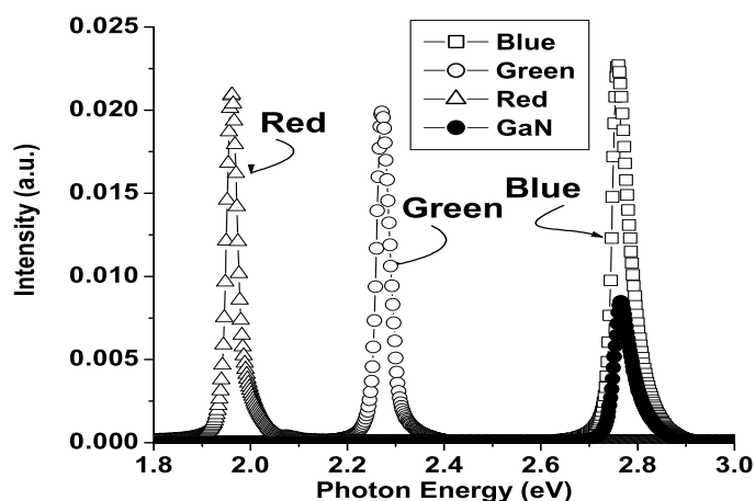
Figure 8. Intensity spectra of red, green, and blue InGaN QWs in the white LED design using AlInGaN as barrier material. Solid dots represent spectrum for typical blue LED.
