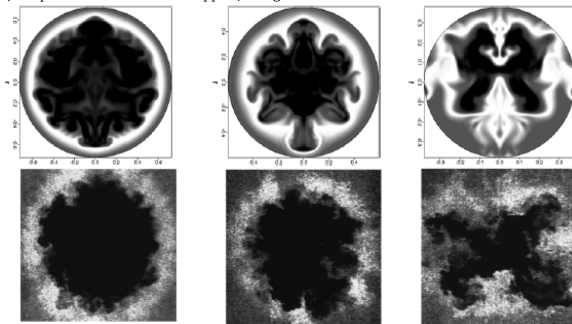
Figure 1. End-views of contours of instantaneous local Mach number (top) at Re_D=100,000 and M=2.46 , compared with visualizations from experiment by Bourdon and Dutton (bottom) at Re_D=3,300,000 and
