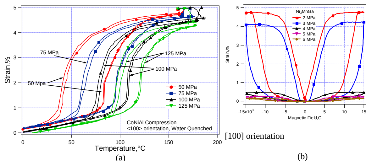
Figure 7. (a) Strain vs. temperature response of a new CoNiAl alloy under different constant stress levels showing more than 4% shape memory strain, shrinkage in hysteresis as a function of stress and complete recoverability. (b) Strain vs. magnetic field response of Ni 2 MnGa demonstrating very large MFIS (more than 4.5%), the coupled effect of magnetic/stress fields on strain level, hysteresis, the field at which reorientation starts and stored energy are notable.
