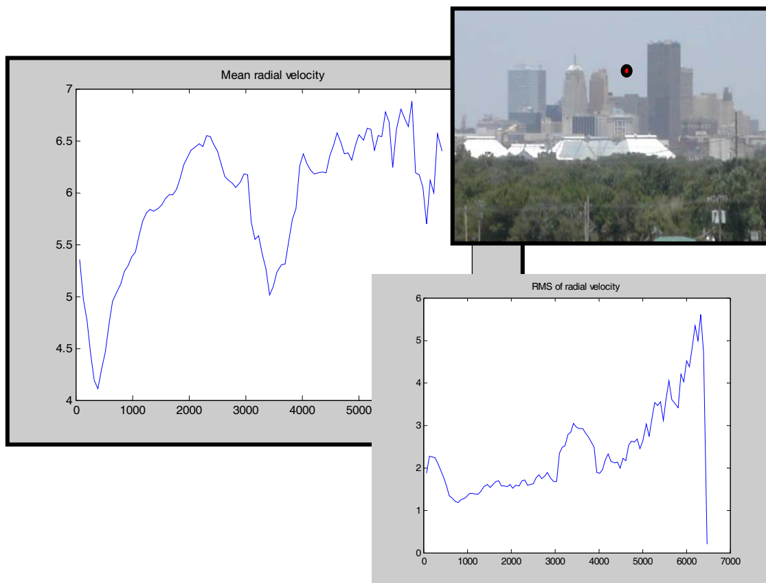
Figure 6. Mean radial wind speed and rms velocity fluctuation in airflow entering and transecting the Oklahoma City central business district.
