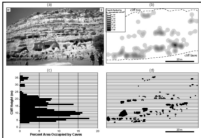
Figure 2. Results of geospatial analysis of caves exposed along the cliffs of Matala, Crete. (a) Photograph of caves; (b) Cave density map; (c) Profile of cave area distribution; (d) Sketch of caves. Note linear trends of high cave density in (b) and major peaks in cave area in (c) that identify specific horizons of enhanced cave development. These horizons can be mapped and selected for closer scrutiny by ground forces
