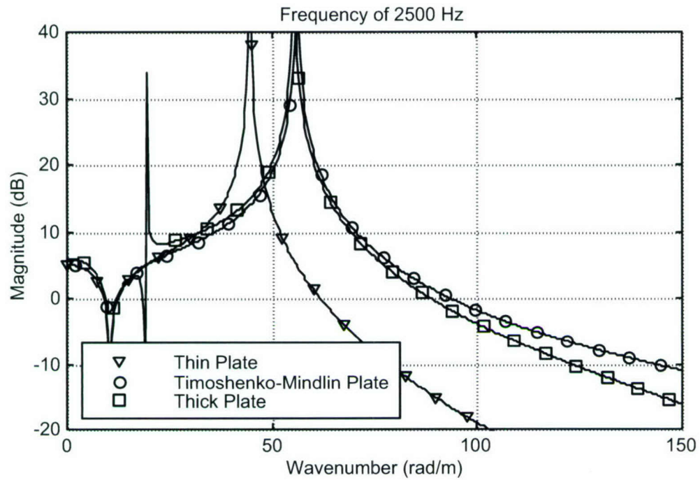
Figure 9. Normalized Velocity Versus Wavenumber Without Masses at 2.5 kHz
