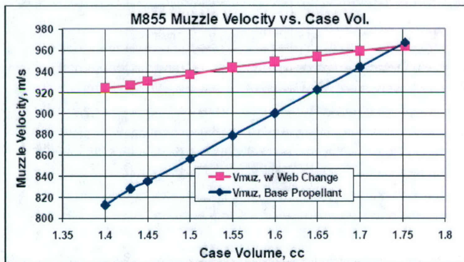
Figure 17 Muzzle velocity versus case volume at 450 MPa chamber pressure
