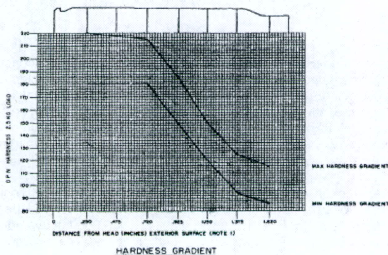
Figure 2 Surface hardness gradient of M855 brass cartridge case
