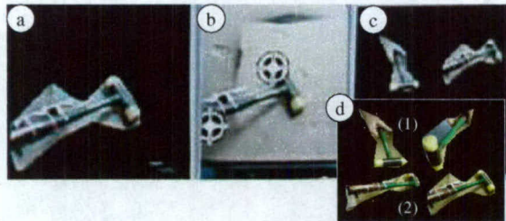
Fig. 9. Human-robot skill transfer, from an on-line experiment. a) Hammer visual segmentation by having the robot hammering on a table. (b) Tracking multiple objects – the robot grip and the hammer – based on the Lucas-Kanade pyramidal tracker algorithm. (c) It shows two segmentations. One first obtained from human demonstration (on the left). The second (on the right), was segmented from robot actuation, and it was recognized as belonging to the same category as the first (otherwise it would not appear on the same window during the experiment). d) Several segmentations obtained by human demonstration and by the robot's experimental manipulation.
