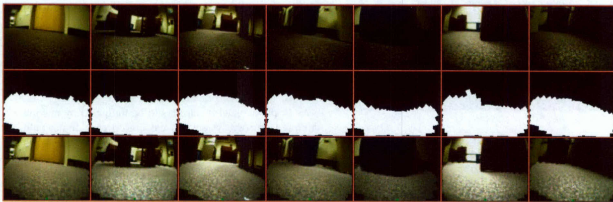
Figure 5. Floor segmentation in action. The top row shows original images, the second row shows masks corresponding to the floor, and the bottom row overlays the two.
