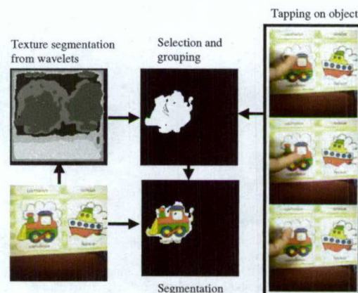
Fig. 10. Texture segmentation of an image and grouping of texture clusters. The method is applied successfully for a case in which the grouping for color regions fails, due to color similarity with background (the white color).
