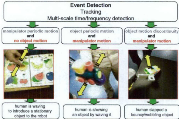
Fig. 2. Image objects are segmented differently according to scene context. The selection of the appropriate method is done automatically. After detecting an event and determining the trajectory of periodic points, the algorithm determines whether objects or actuators are present, and switches to the appropriate segmentation method.
