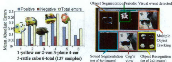
Fig. 13. (left) Statistical results for the segmentation of the objects shown. Results shown in graph (6) correspond to data averaged from a larger set of objects on the database (right) Visual segmentations are used to initialize a multi-target tracking algorithm, to keep track of the objects' positions. An object recognition algorithm, which matches templates based on color histograms, is also shown running.
