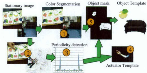
Fig. 3. A standard color segmentation algorithm computes a compact cover for the image. The actuator's periodic trajectory is used to extract the object's compact cover – a collection of color cluster sets.
