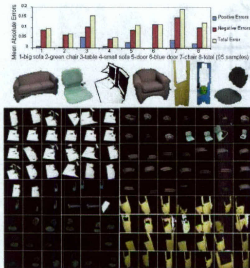
Fig. 4. Statistics for the furniture items (a set of segmentation samples is also shown). Errors are given by (template area - object's real visual appearance area)/(real area). Positive errors stand solely for templates with larger area than the real area, while negative errors stand for the inverse. Total errors stand for both errors. The real area values were determined manually. A chair is grouped from two disconnect regions by merging temporally and spatially close segmentations.
