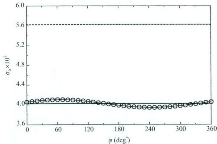
FIGURE 10. Effect of longitudinal admittance on the second-mode stability: F = 1.2385 \times 10^{-4} , R = 2095 ; ---, solid wall; —, A_y = -1 , A_x = 0 ; \circ , A_y = -1 , A_x = \exp(i\phi \pi/180) .
