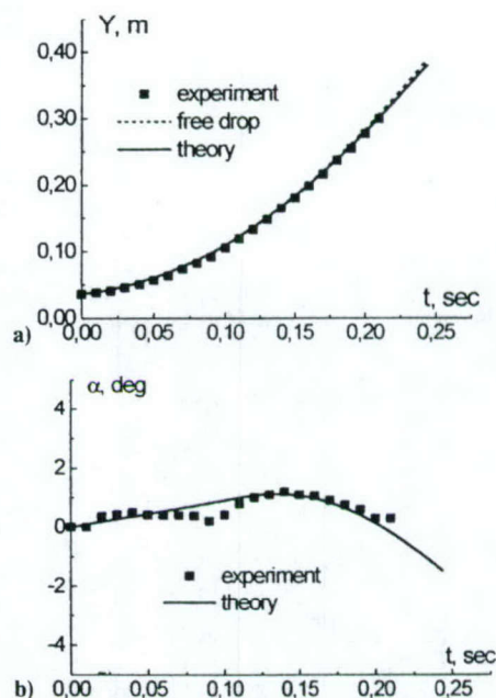
Fig. 3 Model B4N2, U_\infty = 62.3 m/s, Y_0 = 1.42 in. (0.0361 m), \alpha_0 = 0 deg, V_0 = 8 in./s (0.2032 m/s), and \omega_0 = 9 deg/s.
