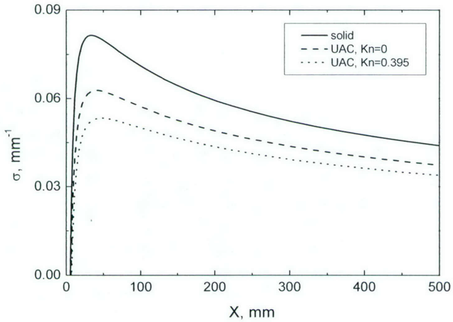
Fig. 2 Rarefaction effect on the UAC performance; T_w = T_{ad} , Re_1 = 2 \times 10^7 \text{ m}^{-1} , M_e = 5.3 , T_e = 56.4 \text{ K} .
