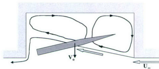
Fig. 2 Flow scheme for the store dropping inside a shallow cavity.
