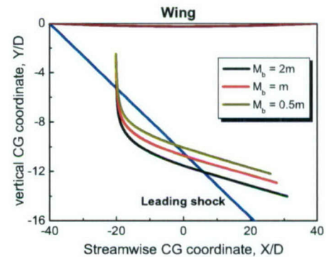
Fig. 8 Effect of the body mass on the CG trajectory at the interaction with the leading shock. X_0 = -20D , Y_0 = -2.5D , V_0 = -5 m/s.
