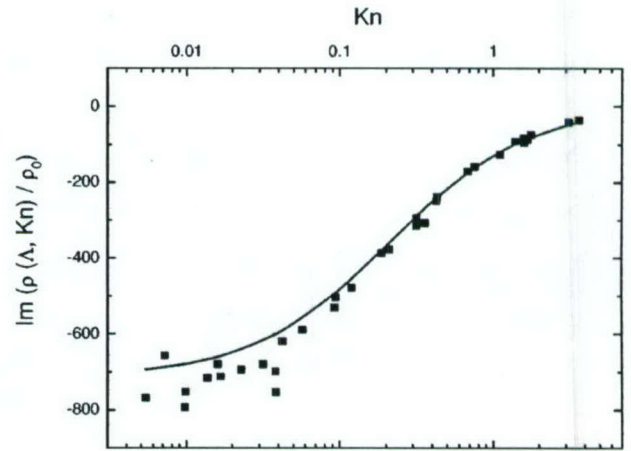
FIG. 6. Comparison of theoretical predictions (solid lines) for the normalized imaginary part of dynamic density at |\Lambda|=10^{-1} , \alpha_u=0.9 with those resulted from experimental data 27 for flow of argon in the square tube of 2.5-mm cross-section side and 305-mm length (squares).
