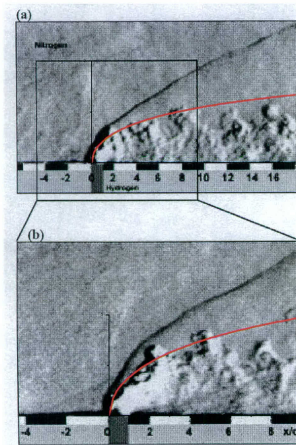
Figure 4. Comparison of the theoretical solution (7) (red line) with simultaneous schlieren image of hydrogen injection into supersonic cross-flow; 2 M = 3.5 , T^* = 1300 K, p^* = 0.32 psi, U_\infty^* = 2420 m/s; the jet-to-freestream momentum flux ratio \alpha = 2 .
