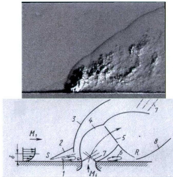
Fig. 12. Upper panel : Schlieren image of the normal under-expanded hydrogen injection into supersonic cross-flow from Ref. 43; Lower panel : schematic of the flow pattern (from Ref. 44): 1 - separation bubble upstream the jet exit; 2 - shock due to upstream separation at the point S ; 3 - bow shock induced by the jet; 4 - Mach disc; 5 - separation bubble downstream from the slot; 6 - expansion waves; 7 - shock induced by the jet reattachment R ; M_1 - freestream Mach number; M_j - Mach number of the out-flowing jet.
