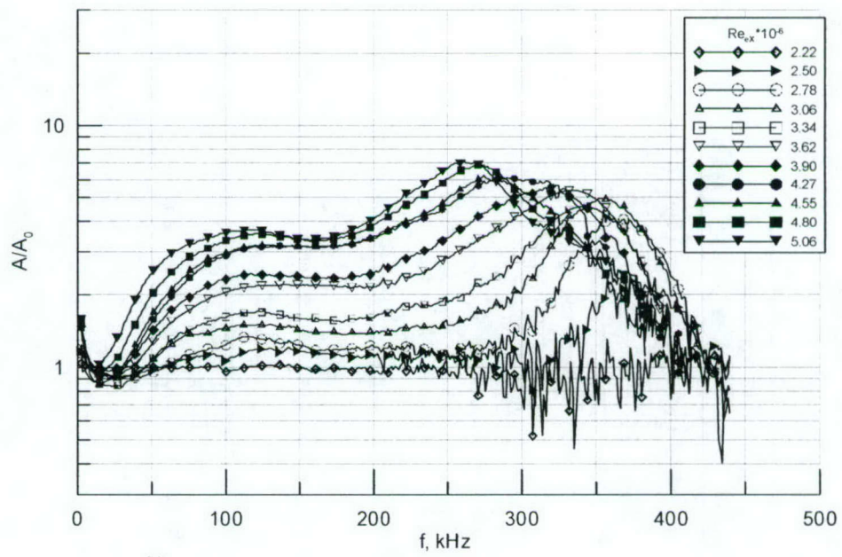
Fig. 6 Normalized natural-disturbance spectra on the solid (a) and porous (b) sides at various Re_x .
