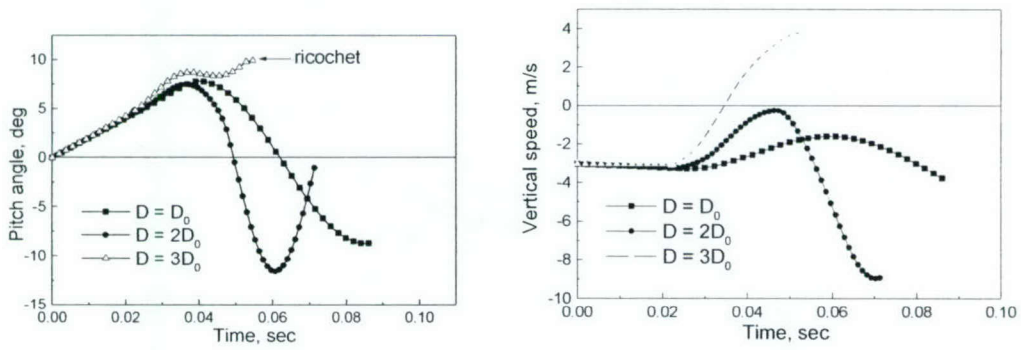
c) Pitch angle histories.
