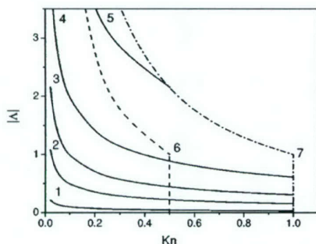
FIG. 2. The |\Lambda| - Kn diagram of the regimes of validity of the asymptotic theory. Isolines 1-5 correspond to constant ratios L_p/\lambda: 1-L_p/\lambda=10^{-4} , 2-L_p/\lambda=2.5 \cdot 10^{-3} , 3-L_p/\lambda=10^{-2} , 4-L_p/\lambda=0.04 , and 5-L_p/\lambda=0.25 . The dashed curve 6 restricts the parameter plane by Kn < 0.5 in the low-frequency range and by Kn|\Lambda| < 0.5 in the high-frequency range, respectively. The dash-and-dot line 7 does the same for the corresponding restrictions Kn < 1 and Kn|\Lambda| < 1 .
