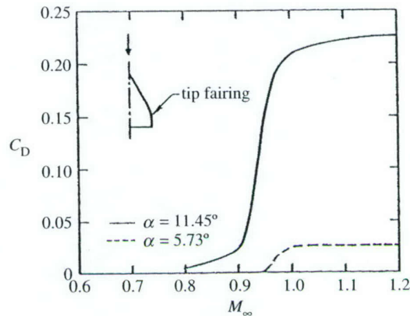
Figure 2. Drag rise due to lift characteristics of model fighter platform.
