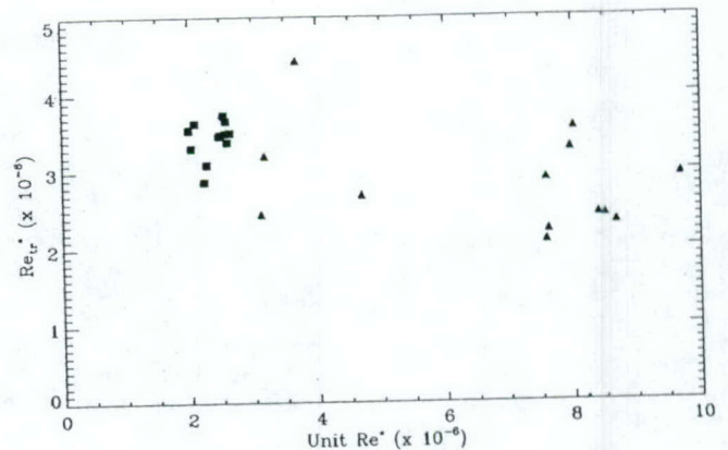
Fig. 10 Reynolds number Re_{tr}^* vs Unit Re^* showing that unit Reynolds number effect was not observed in the transition data on the porous surface.
