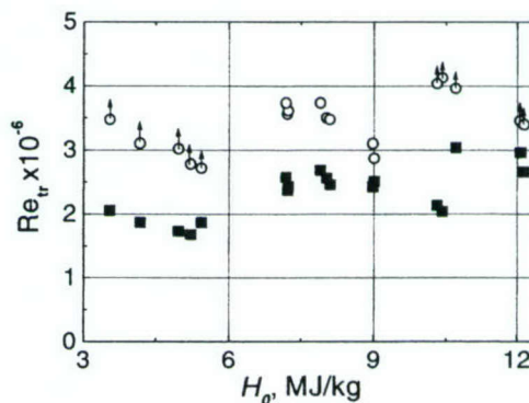
Fig. 10 Transition onset Reynolds number Re_{tr} vs total enthalpy H_0 : ■, solid wall; ○, porous wall; and ○, boundary layer on porous wall is laminar up to the model base.
