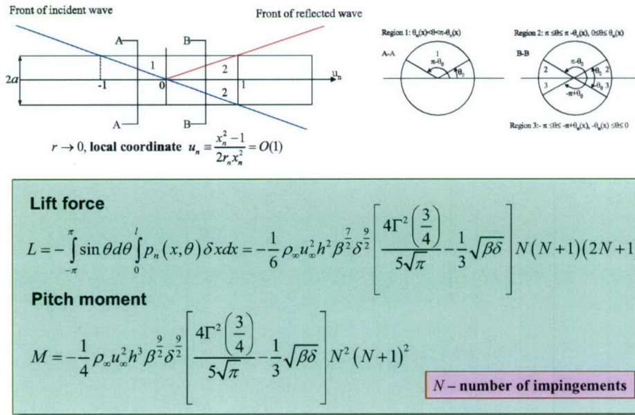
Figure 7. Approximate scheme of local scattering and corresponding analytical solutions for the lift force and pitching moment.
