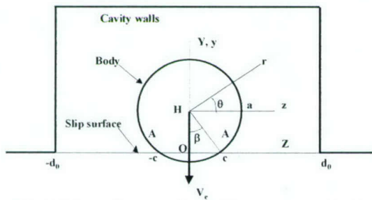
Fig. 2 Flow scheme and coordinate systems: back view.
