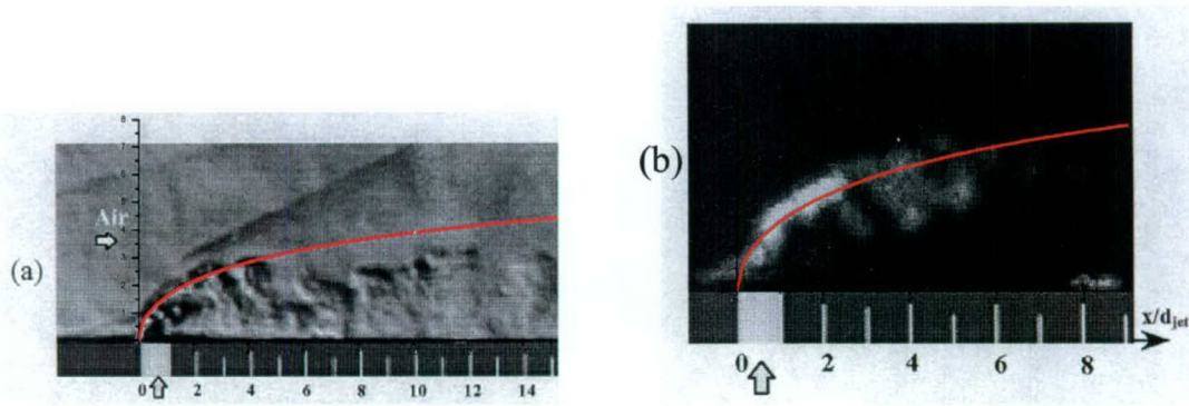
Figure 3. Comparison of the theoretical solution (7) (red line) with simultaneous schlieren (a) and OH-PLIF (b) images of hydrogen injection into supersonic cross-flow; 8 M = 3.46 , T^* = 1300 K, p^* = 0.32 psi, U_\infty^* = 2420 m/s; the jet-to-freestream momentum flux ratio \alpha = 1.4 .
