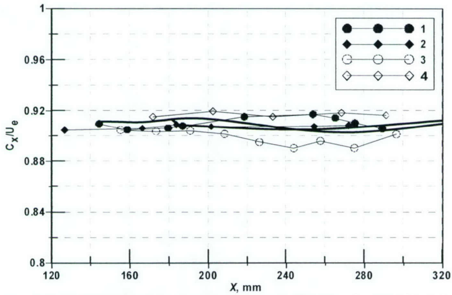
Fig. 8 Phase speeds for artificial disturbances on the porous and solid sides; f = 275 kHz. 1, 2 – solid side; 3, 4 – porous side; black lines – theory.
