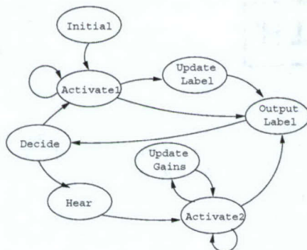
Figure 5: State machine of a Concept behavior.
