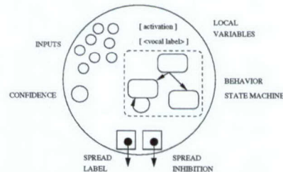
Figure 3: Representation of a single protoverbal behavior.
