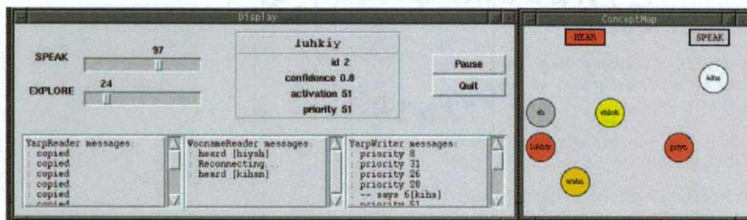
Figure 8: Partial screenshot of an interaction. ConceptMap on the right shows current protoverbal behaviors colored by their priority value. Details of winning behavior also in the main window.
