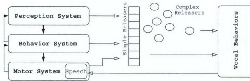
Figure 4: Control and data flow between vocal and other behaviors in Kismet's architecture. Dark arrows indicate combined control and data flow between old components of the architecture. Light arrows follow the data flows only.
