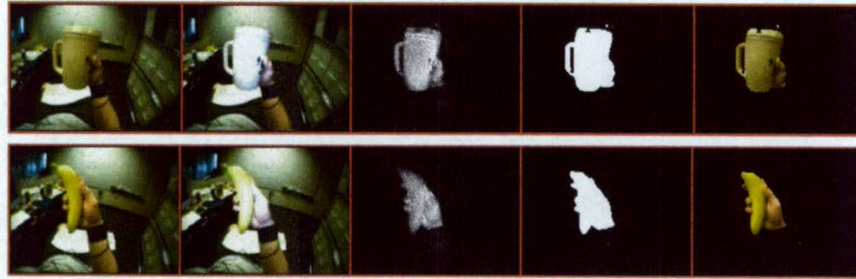
Fig. 6. The system currently achieves segmentation by active sensing. When the wearer brings an object up into view (first column), an oscillating light source is activated (second column). The difference between images (third column) is used to compute a mask (fourth column) and segment out the grasped object and the hand from the background via a simple threshold.(fifth column).
