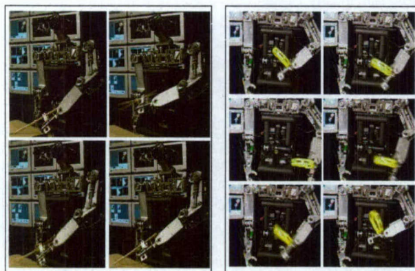
Fig. 6. The humanoid robot Cog playing two musical instruments – a drum (left) and a tamborine (right), after tuning of the neural oscillators. The robot first reaches the instrument using a Sliding Modes Controller [3].
