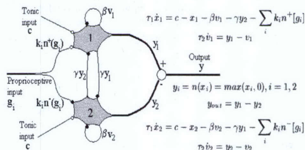
Fig. 1. Matsuoka neural oscillator, composed by two inhibiting neurons.
