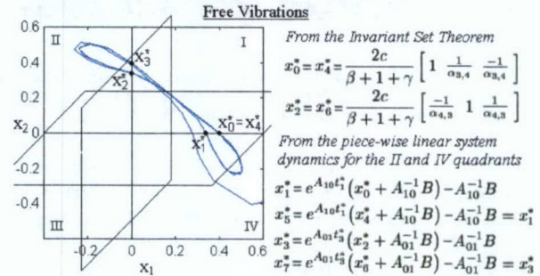
Fig. 5. Two surface sections transverse the flow of the neural oscillator at x_1 = 0 and at x_2 = 0 .
