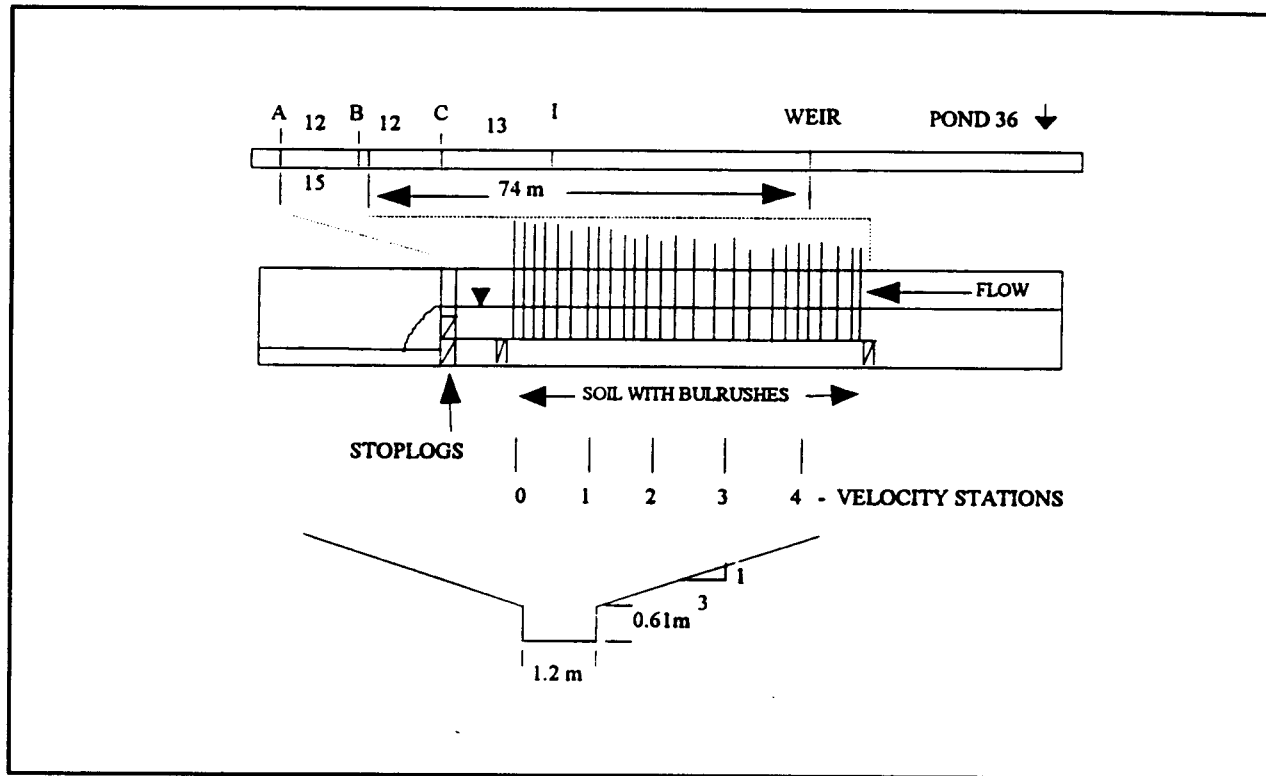
Figure 2. Schematic View of the Lewisville Aquatic Ecosystem Research Facility Test Channel showing test set up and sampling/measurement locations
