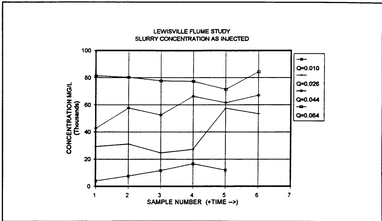
Figure 5. Sediment Concentration of Injected Sediment Slurry
