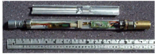
Figure II-6. Example of a Downhole Photoionization Detector (PID).
