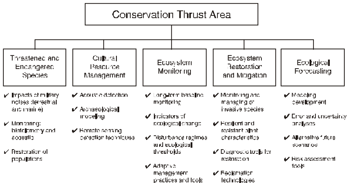
Figure III-6. Conservation Taxonomy.
