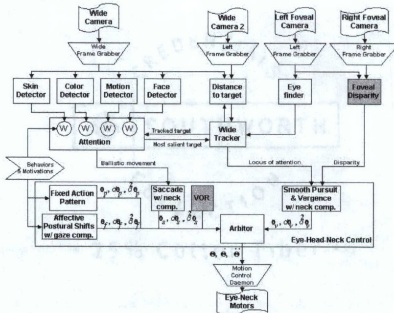
Fig. 13. Organization of Kismet's eye/neck motor control. Many cross level influences have been omitted. The modules in gray are not active in the results presented in this paper.
