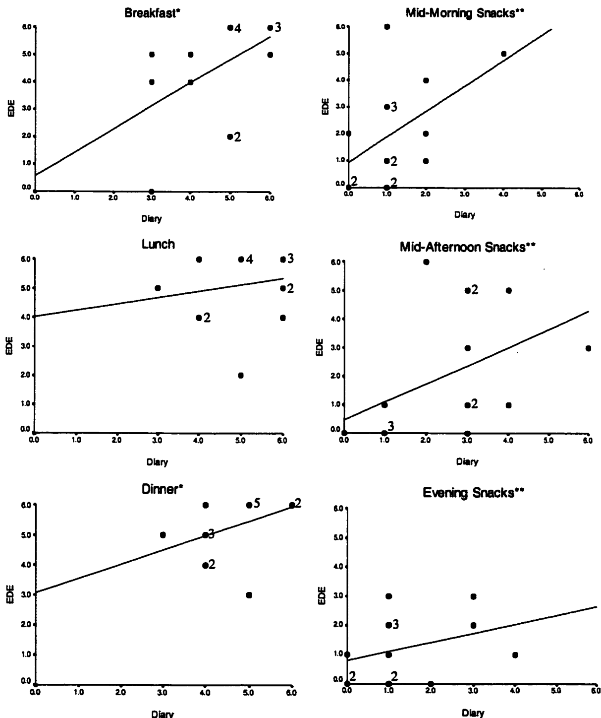
Figure 4. Comparisons of normals' responses for each meal on the EDE vs. the diary. The line represents the linear regression fit. Overlapping data points are represented by a number indicating the number of multiple responses at that point.
