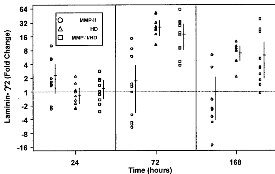
Figure 28. Effect of MMP-2/MMP-9 Inhibitor II (Inhibitor II) on Laminin- \gamma 2 mRNA Levels. Fold change in laminin- \gamma 2 mRNA levels in mouse ear skin pretreated with II only (circles), HD-exposed only (triangles), and pretreated with Inhibitor II and then HD-exposed (squares) at 24 h, 72 h, and 168 h post-exposure. Individual data points are indicated by the shapes. The horizontal dashes represent the geometric mean and the vertical lines represent the 95% confidence intervals.
