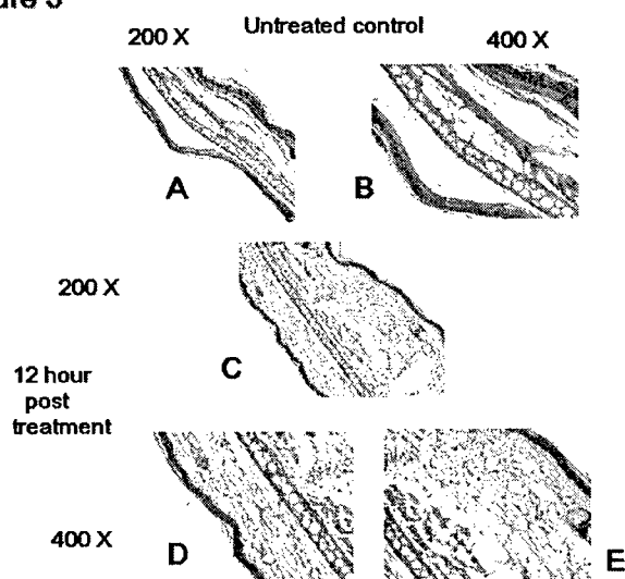
Figure 3. H & E staining from untreated (A and B) and 12 h post-HD-treated (C-E) mouse ear biopsy samples. Inner ear (treated) is to left and outer ear to right. Magnification either 200 X or 400X.
