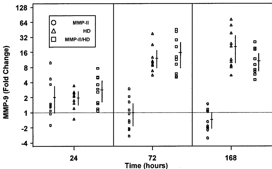
Figure 27. Effect of MMP-2/MMP-9 Inhibitor II (Inhibitor II) on MMP-9 mRNA Levels. Fold change in MMP-9 mRNA levels in mouse ear skin pretreated with Inhibitor II only (circles), HD-exposed only (triangles), and pretreated with Inhibitor II and then HD-exposed (squares) at 24 h, 72 h, and 168 h post-exposure. Individual data points are indicated by the shapes. The horizontal dashes represent the geometric mean and the vertical lines represent the 95% confidence intervals.
