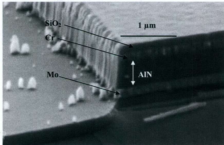
Figure 3.13: \text{CF}_4/\text{O}_2 overetch (25%) of Mo showing no observable undercut.
