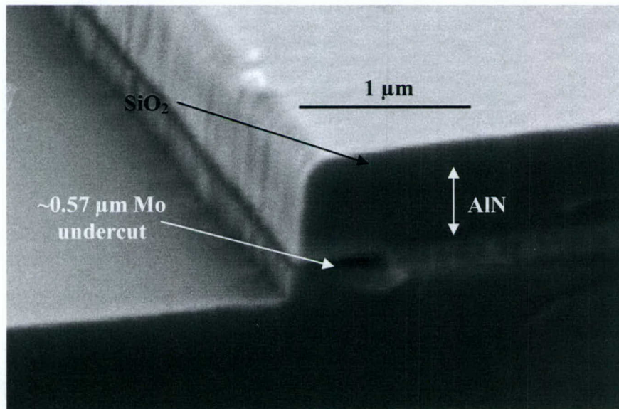
Figure 3.8: Undercut effects of ~2.5 minute overetch (250%) of Mo with Cl 2 LO recipe.
