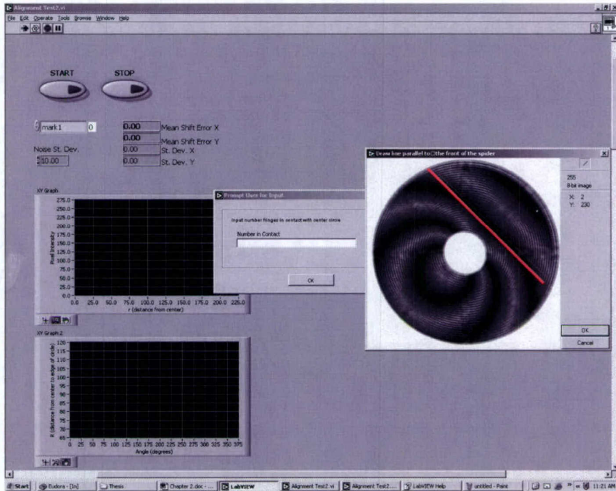
Figure 2.15: The operator draws a line parallel to front of “spider” and inputs “2” as the number of dark fringes passing through the center point.
