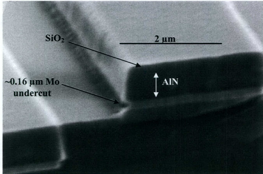
Figure 3.7: Undercut effects of ~2.5 minute overetch (250%) of Mo with Cl 2 /Ar LO recipe.
