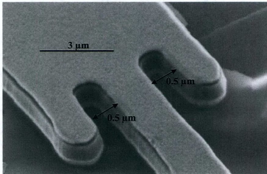
Figure 4.4: Angle view of 0.5 μm notches at the resonator-tether interface.
