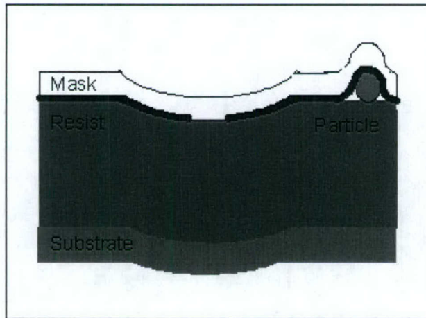
Figure 2.3: A flex mask is able to conform around substrate shape variations. 1
