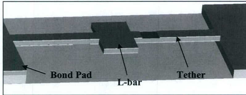
Figure 1.1: Schematic of suspended MEMS L-bar resonator. 1
