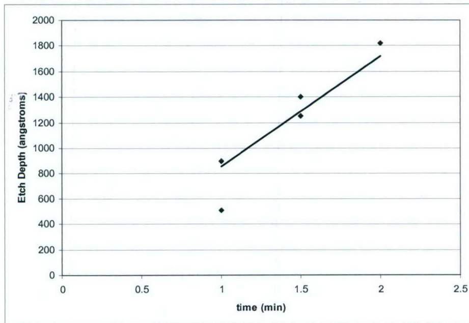
Figure C.1: Etch depth vs. time of PECVD SiO 2 in F-based plasma
