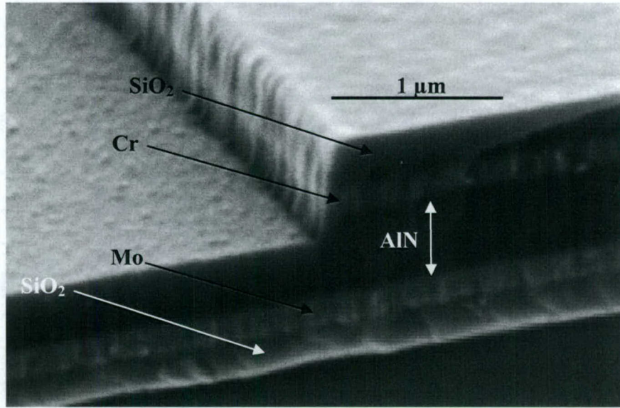
Figure 3.16: Partial AlN etch: After 2 minute 30 second Cl 2 /O 2 LO etch and 1 minute Cl 2 /Ar LO etch.
