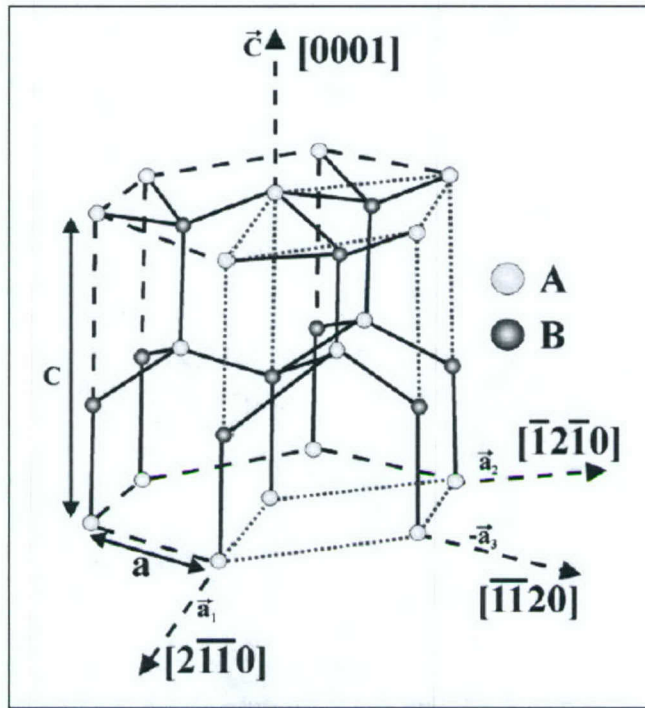
Figure 3.1: Polar wurtzite crystal structure [21].
