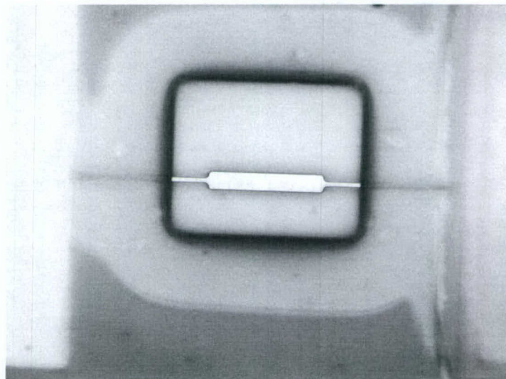
Figure 4.2: Perfectly aligned ( \sim \pm 50 nm in x-direction) release etch window.
