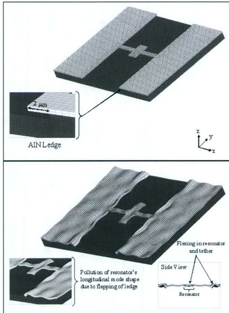
Figure 1.6: Top – Profile of the free hanging ledge produced by \text{SiO}_2 undercutting; Bottom – Simulated “flapping” motion of the ledge which pollutes the resonator’s longitudinal mode shape [7].
