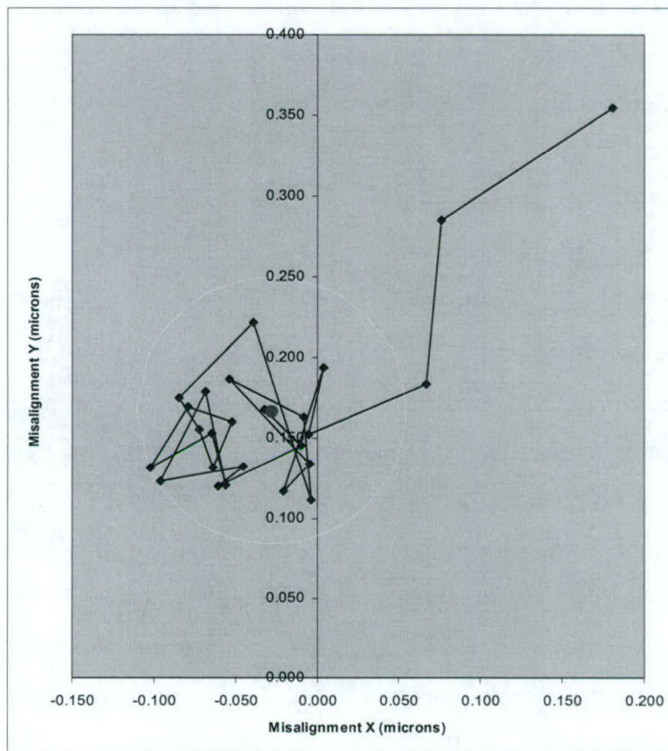
Figure 2.22: 25 contact/release cycles in relation to their standard deviation radius.
