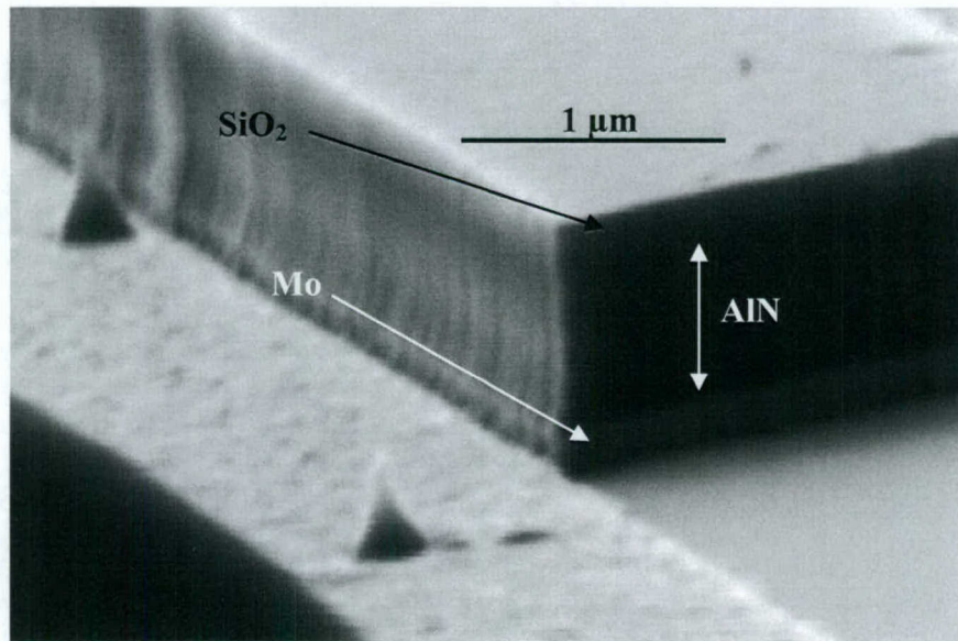
Figure 3.11: AlN etch with Cl 2 /Ar LO recipe.
