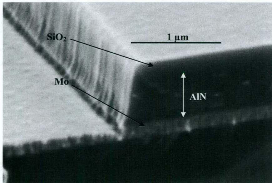
Figure 3.12: AlN etch with Cl 2 LO.
