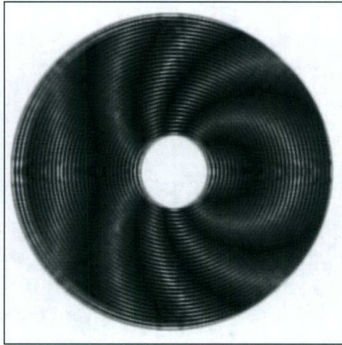
Figure 2.8: Simulated misalignment with marks of equally-pitched circular gratings. The pitch of the gratings is 2\ \mu\text{m} , thus it can be inferred from the image that there is a misalignment of about 4\ \mu\text{m} .
