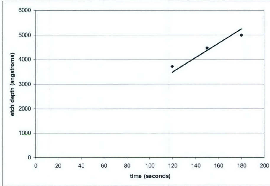
Figure 3.10: Etch rate of AlN with Cl 2 LO recipe (1750 Å/min).
