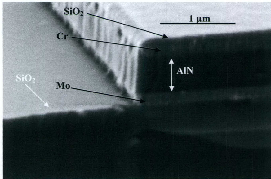
Figure 3.19: Mo etch: After 2 minute 30 second Cl 2 /O 2 LO etch, 4 minute Cl 2 /Ar LO etch, and 2 min 30 second CF 4 /O 2 etch.
