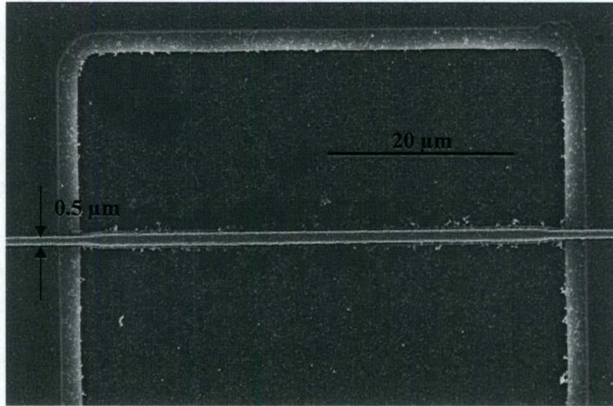
Figure 4.5: 1 \mu\text{m} x 50 \mu\text{m} resonator with 0.5 \mu\text{m} tethers.
