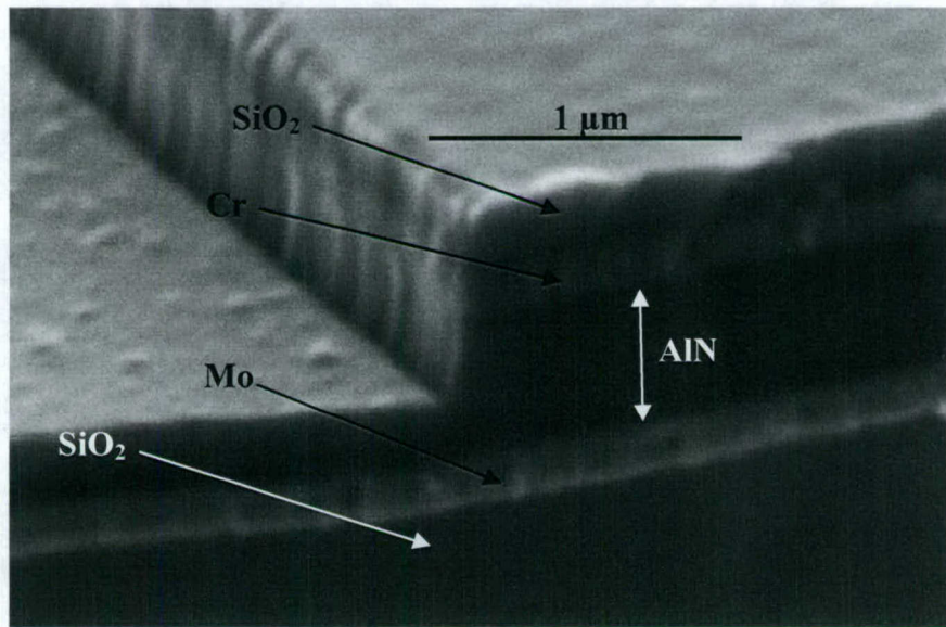
Figure 3.17: Partial AlN etch: After 2 minute 30 second Cl 2 /O 2 LO etch and 2 minute 15 second Cl 2 /Ar LO etch.
