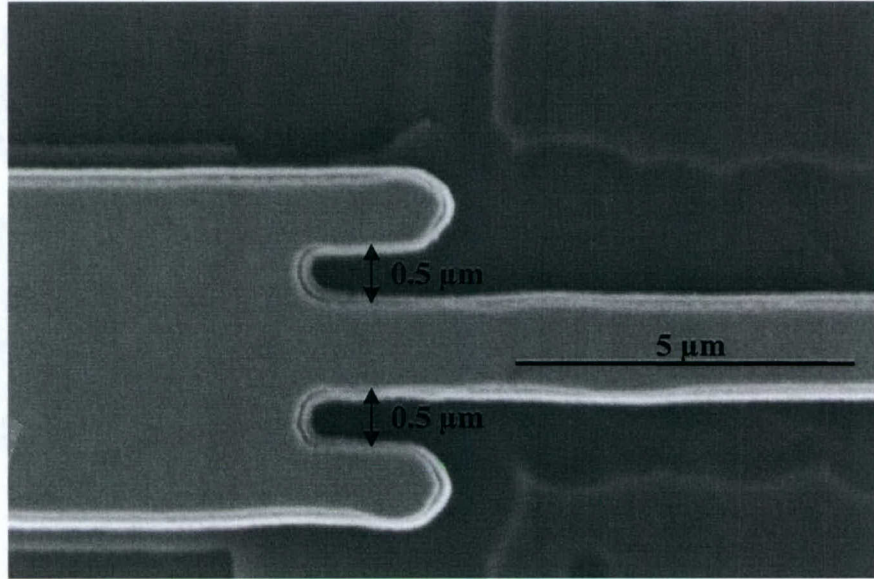
Figure 4.3: Top view of 0.5 μm notches at the resonator-tether interface.
