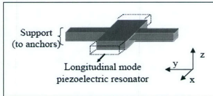
Figure 1.2: Resonator's intended mode of operation. 1
