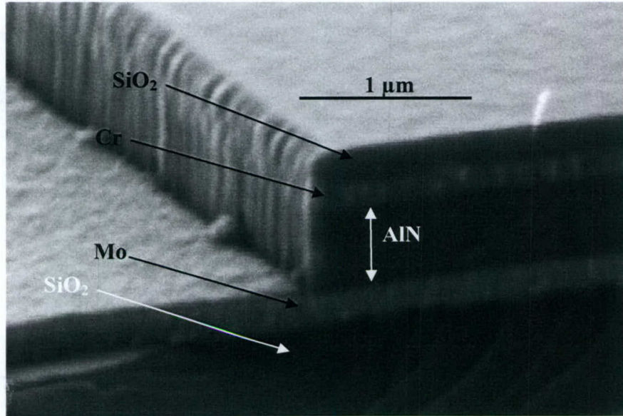
Figure 3.18: AlN etch: After 2 minute 30 second Cl 2 /O 2 LO etch and 4 minute Cl 2 /Ar LO etch.
