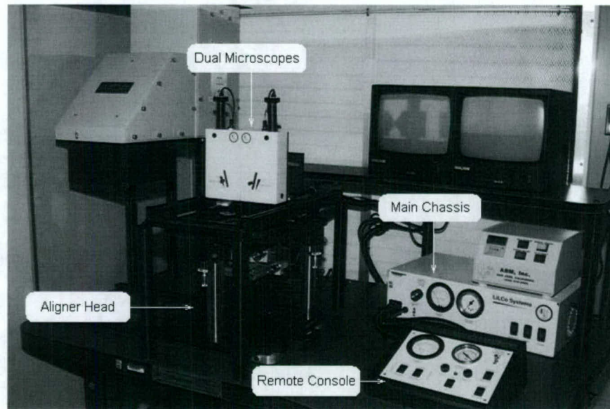
FIGURE 2.4: CCL system layout. 1
