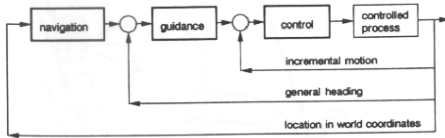
Figure 38: Supervisory Control (from [Sheridan 93])
