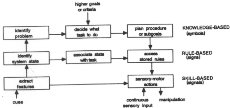
Figure 39: Multiple Levels of Human Reasoning (from [Sheridan 93])
