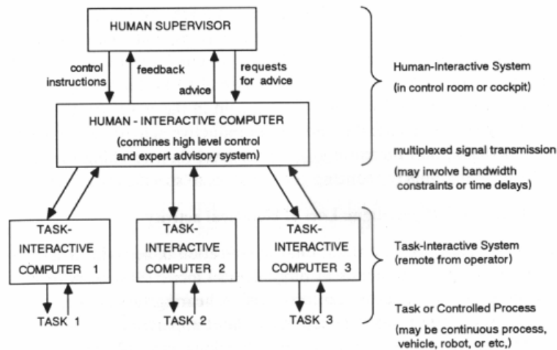
Figure 40: Control of multiple computers/robots concurrently (from [Sheridan 93])
