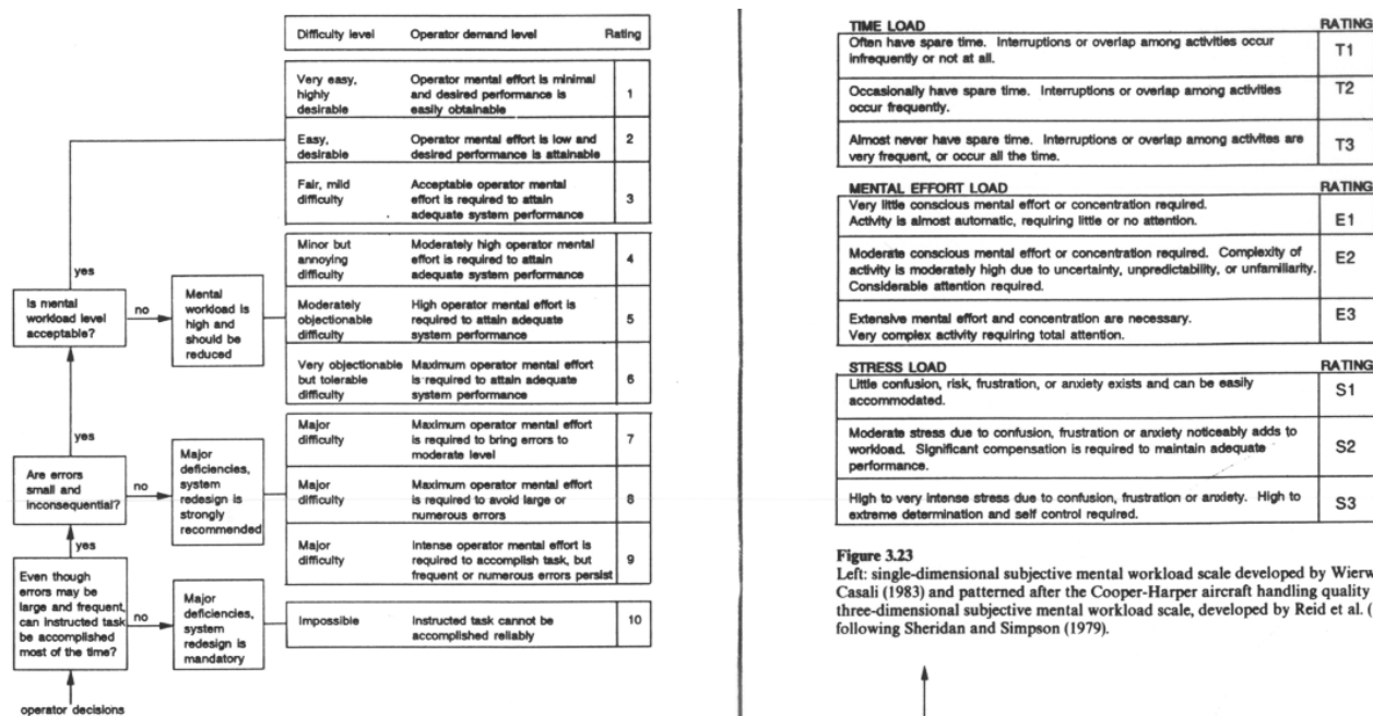
Figure 47: Workload Measurement Rating System (from [Sheridan 93])
