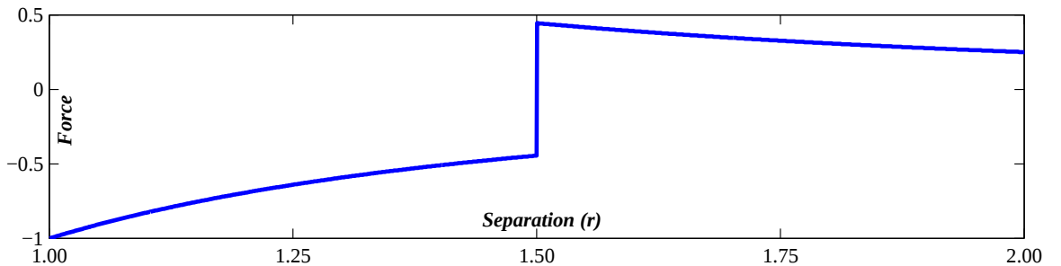
Figure 14.5: Plot of a sample force function used by the AP asset controller, with r_{\text{desired}} = 1.5 and p = 2 .
