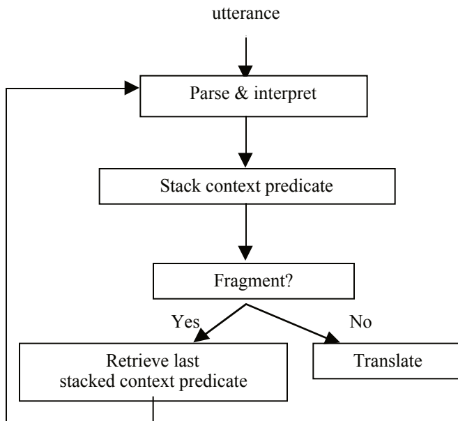
Figure 2: Schematic flowchart for obtaining context predicates
