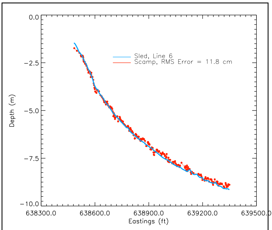
Figure 15: Comparison between USACE sled (blue) and SCAMP hydrographic system profiles obtained from line 6 of survey grid. Large rms error is largely due to the HYPACK®MAX timing problem.
