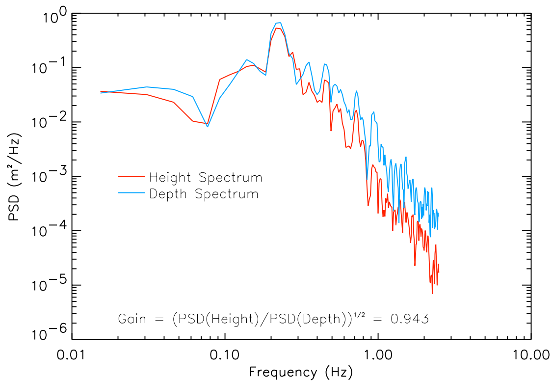
Figure 8: PSDs from GPS antenna height and sounder time series. Relative energy in wave motion band is used to normalize sounder output to local sound speed.
