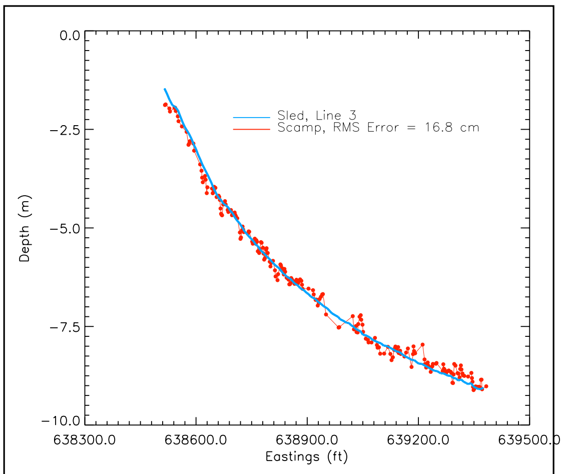
Figure 16: Similar to Figure 15. Residual noise from the HYPACK® timing problem varies with the number of incorrectly positioned time gaps. Here the rms error is near the largest observed, 16.8 cm.
