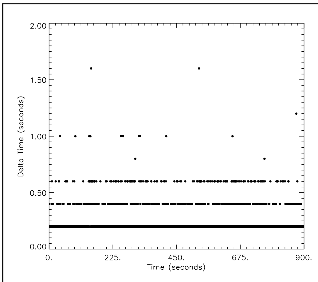
Figure 9: HYPACK delta-t between sequential data points. Reporting rate is 0.2 s. delta-t of 0.4=1 missed GPS update, 0.6=2 missed GPS updates.
