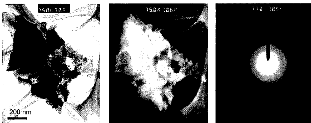
Figure 6 TEM micrographs for as-atomized \text{Al}_{85}\text{Ni}_{10}\text{La}_5 powders ( <25\ \mu\text{m} ): (a) bright filed image, (b) dark filed image, and (c) the selected area diffraction pattern
