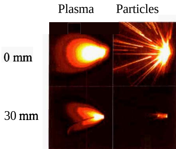
Figure 15: Plasma and Late Time Vaporization divergence in a 1/4"-diameter, 2-electrode MicroPPT firing at 5 J. The curved rod visible in the plasma pictures is an spark plug used to ignite the main discharge.
