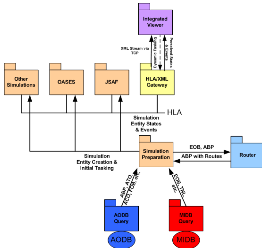
Figure 2.2. JSB-RD Components
