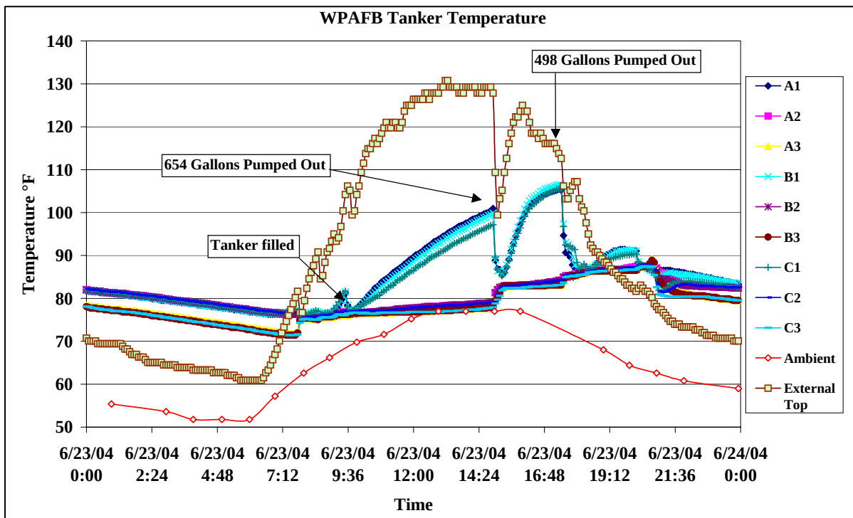
Figure 13: Temperature during activities on July 23 rd WPAFB.
