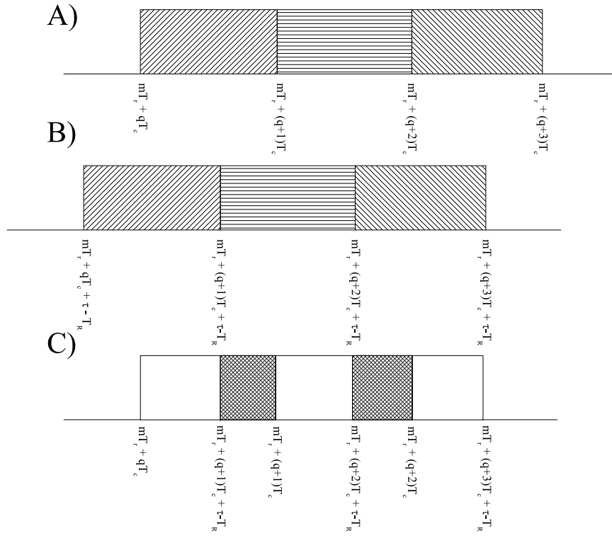
Figure 3.1: The case is when the received chip is matched early. The phase offset are shown by a cross-hatch while the equal phase cases are blank.
