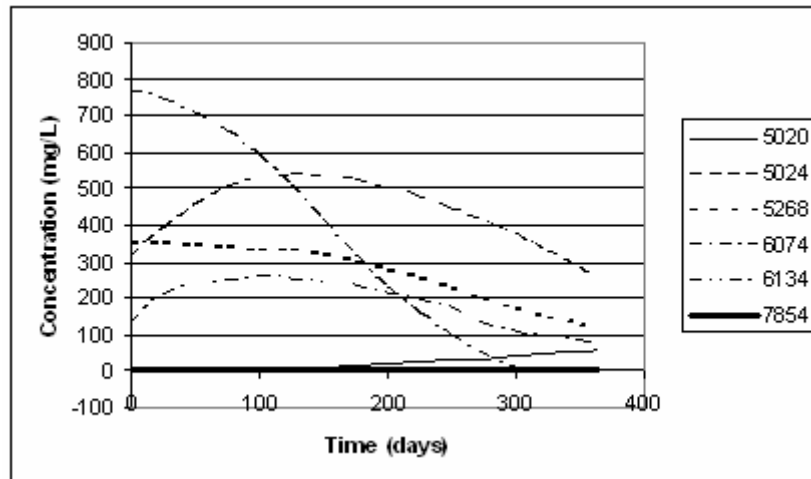
Figure 4.13: Simulated TCE concentrations at pumping wells for scenario four
