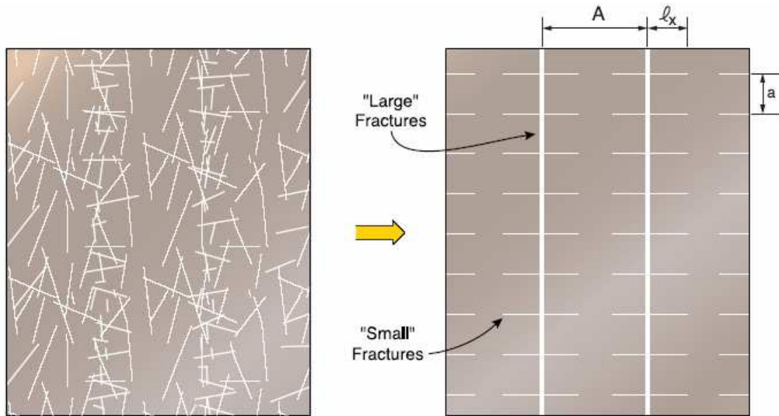
Figure 2.6: Basic conceptualization for triple continuum approximation of a field system (from Wu et al. , 2004)
