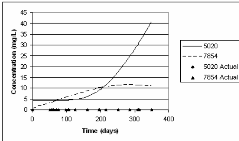
Figure 4.7: Simulated and measured TCE concentrations for pumping scenario two at two toe wells
