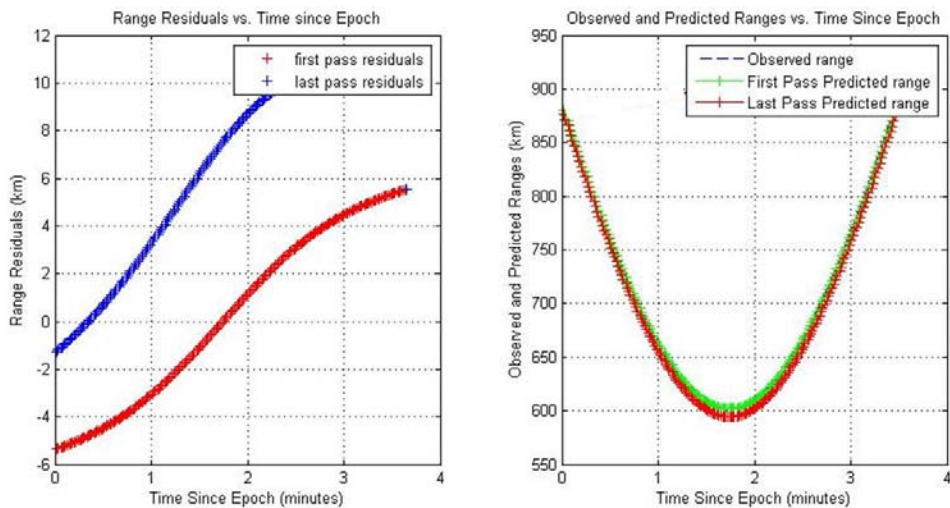
Figure 9 Second iteration residuals and fit in the batch filter
