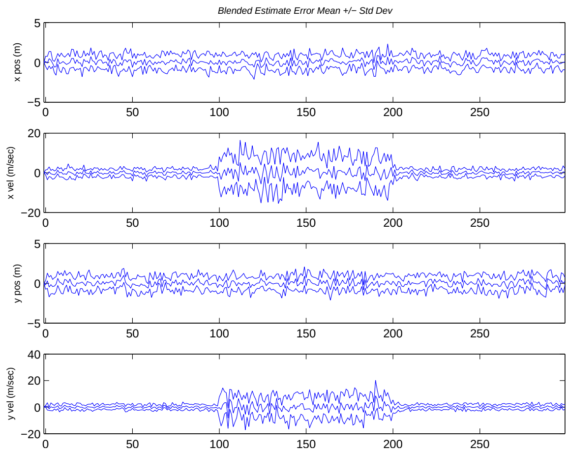
Figure 4.10: Blended estimate for the two-filter system. (Suite 4 vs. Scenario 7: MMAE)
