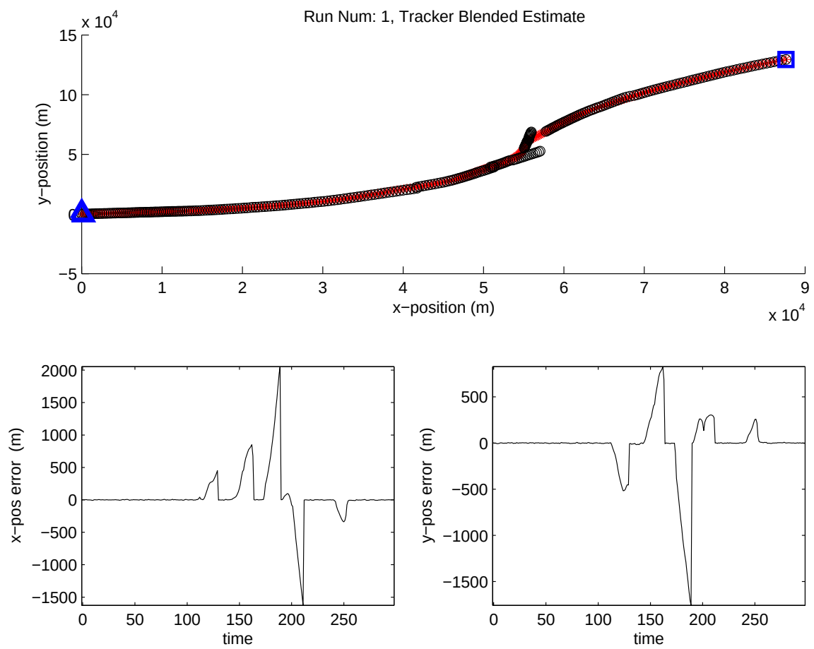
Figure 4.62: Blended output on run number 1. (Suite 4 vs. Scenario 4: MMAE )
