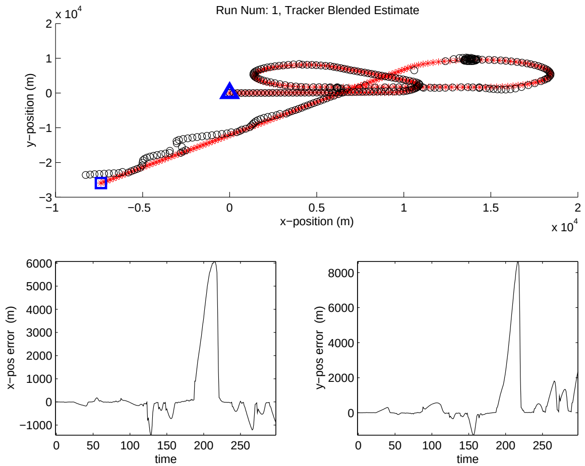
Figure 4.80: IMM Blended estimate for run number 1 in which truth includes three, +3-g TPV maneuvers. (Suite 5 vs. Scenario 5: IMM (Non-Trans. Favor. Markov))
