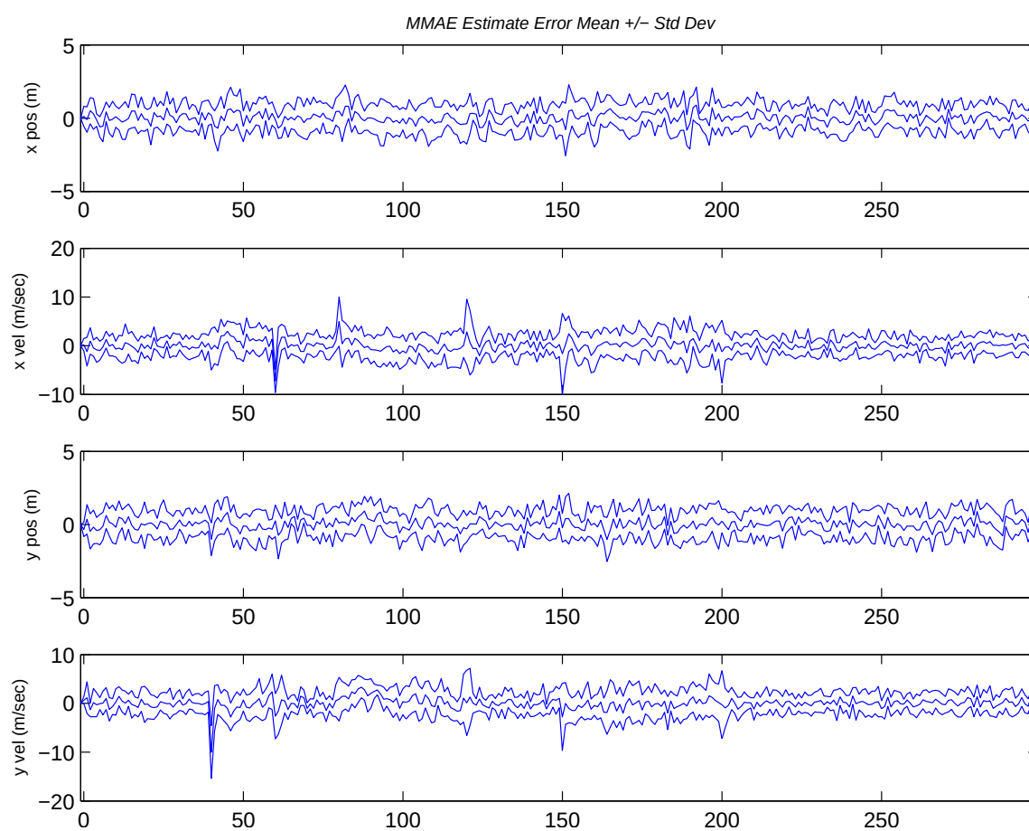
Figure 4.36: Blended estimate. (Suite 6 vs. Scenario 6: MMAE)
