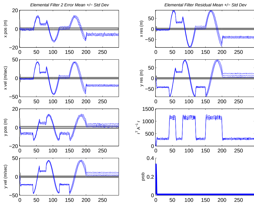
Figure 4.18: Filter 2 output. (Suite 5 vs. Scenario 5: MMAE)
