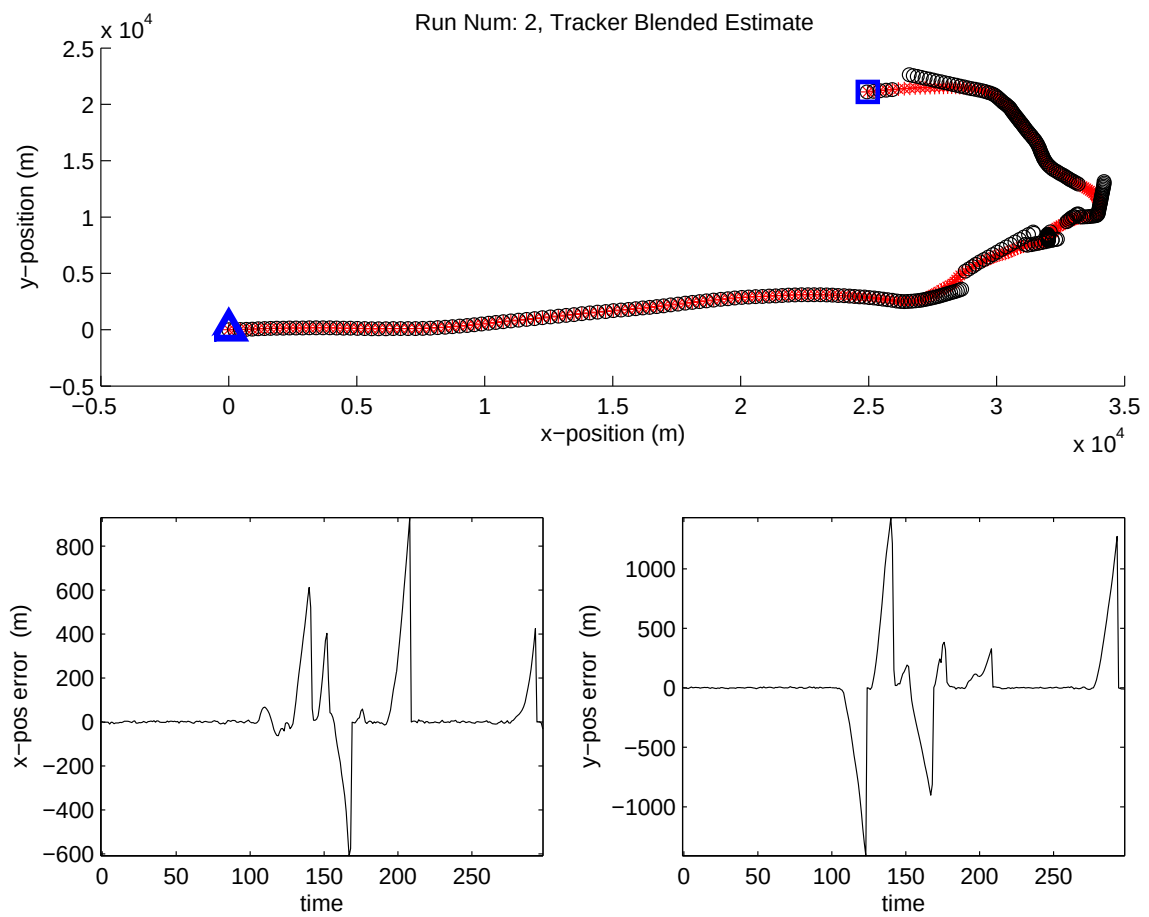
Figure 4.108: Blended solution on Monte Carlo run number 2. (Suite 4 vs. Scenario 4: MMAE)
