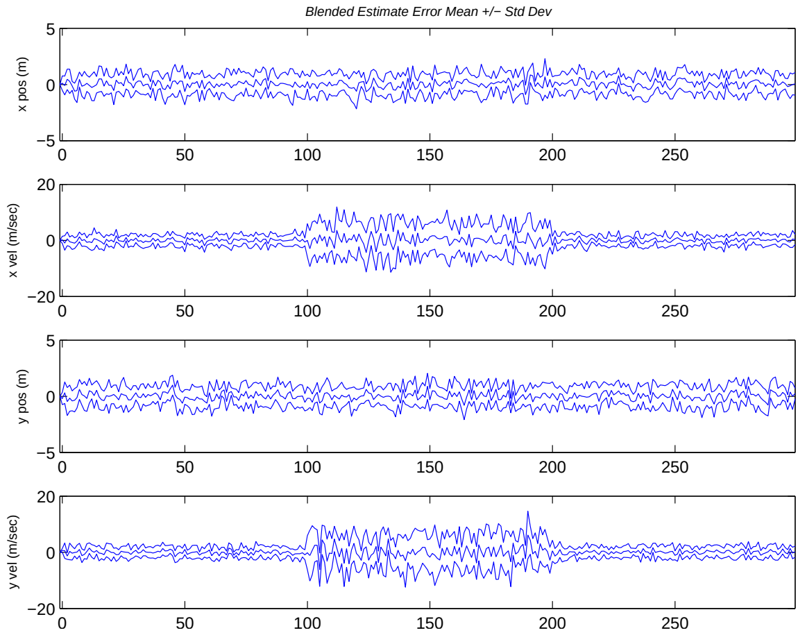
Figure 4.7: Blended estimate for the two-filter system. (Suite 4 vs. Scenario 4: MMAE)
