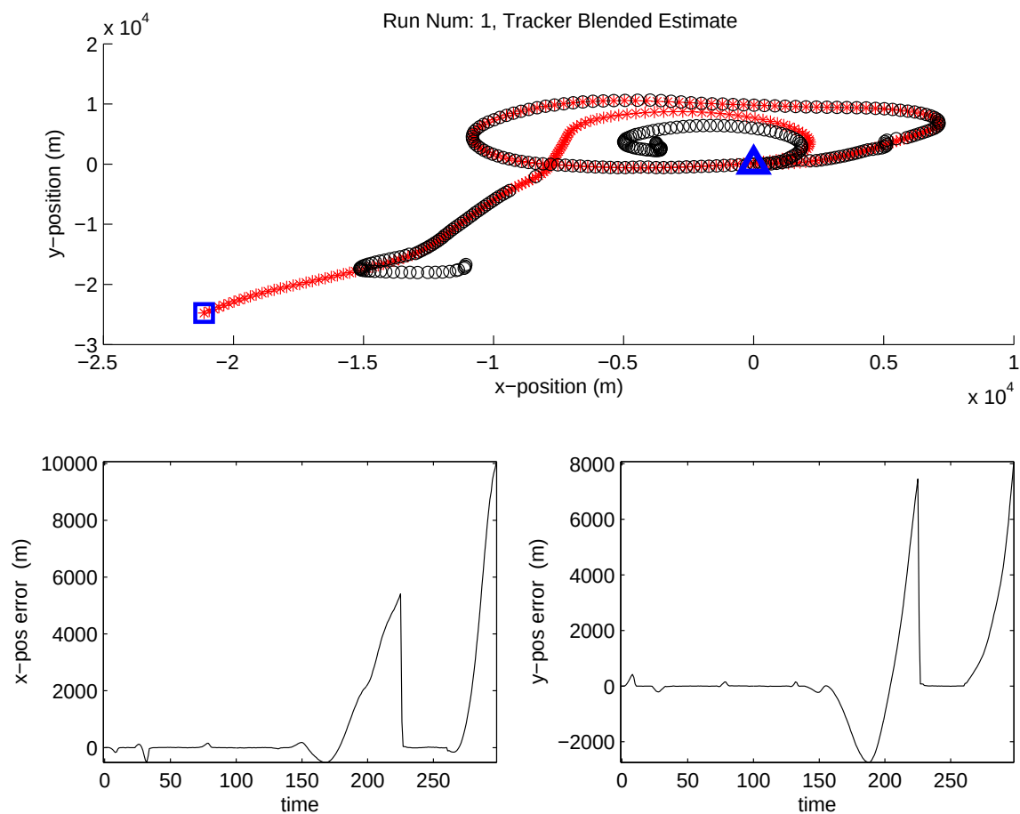
Figure 4.141: IMM Blended estimate for run number 1 in which truth includes three, +3-g TPV maneuvers. (Suite 6 vs. Scenario 6: IMM (Non-Trans. Favor. Markov))
