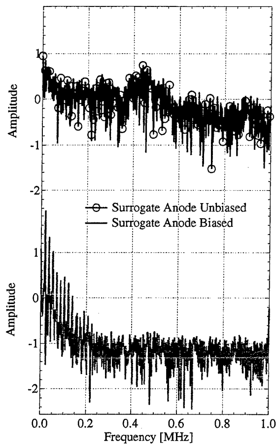
Figure 6. Helium arc voltage fluctuations with and without the surrogate anode biased to draw 13 A. In both cases, the arc discharge current is 10A.
