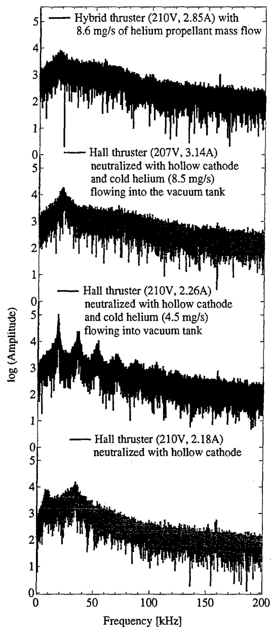
Figure 17. Comparison of Hall discharge current fluctuations with a Hall discharge voltage of 210V.
