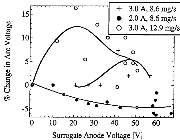
Figure 10. The low-power arcjet voltage change as the surrogate anode voltage increases.
