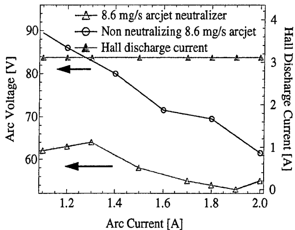
Figure 14. Low-power arcjet (8.6 mg/s mass flow rate) VI curve while neutralizing the Hall thruster (3.1A, 300V).
