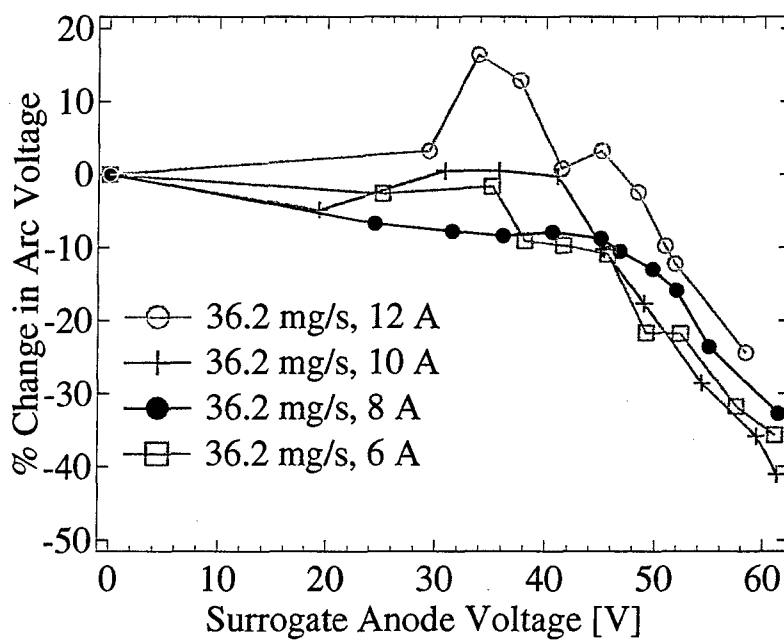
Figure 4. The helium arcjet voltage change as the surrogate anode voltage increases.
