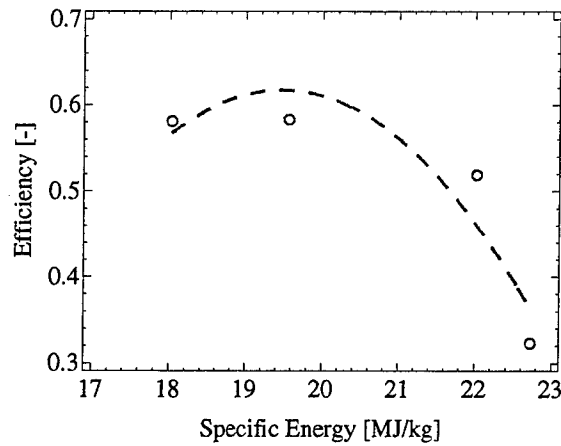
Figure 8. Thrust efficiency of the helium arcjet with a current of 10 A and various mass flow rates.
