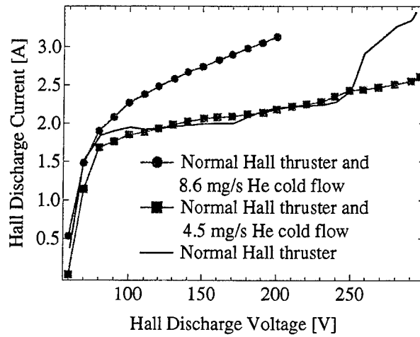
Figure 11. Comparison of the Hall thruster VI curves for different helium flow rates into the vacuum chamber. The normal Hall thruster refers to the Hall thruster neutralized with the hollow cathode.
