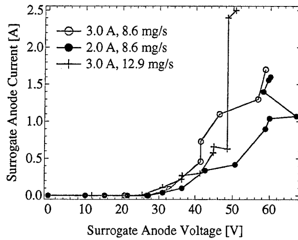
Figure 9. The neutralization current provided by the low-power helium arcjet.
