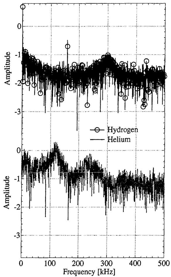
Figure 7. A comparison of the arc voltage power spectra for the hydrogen (13.7 mg/s, 10 A) and helium (36.2 mg/s, 10 A) 1-kW arcjets
