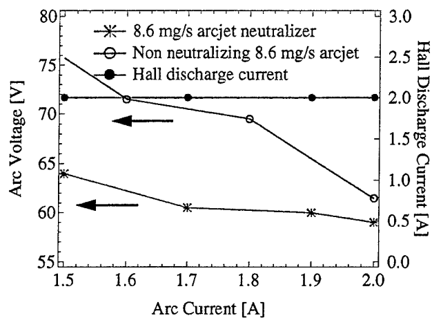
Figure 13. Low-power arcjet (8.6 mg/s mass flow rate) VI curve while neutralizing the Hall thruster (2A, 115V).
