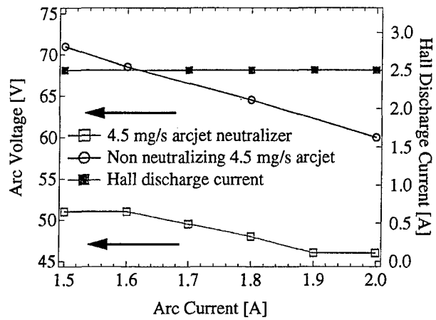
Figure 15. Low-power arcjet (4.5 mg/s mass flow rate) VI curve while neutralizing the Hall thruster (2.52 A, 301 V).
