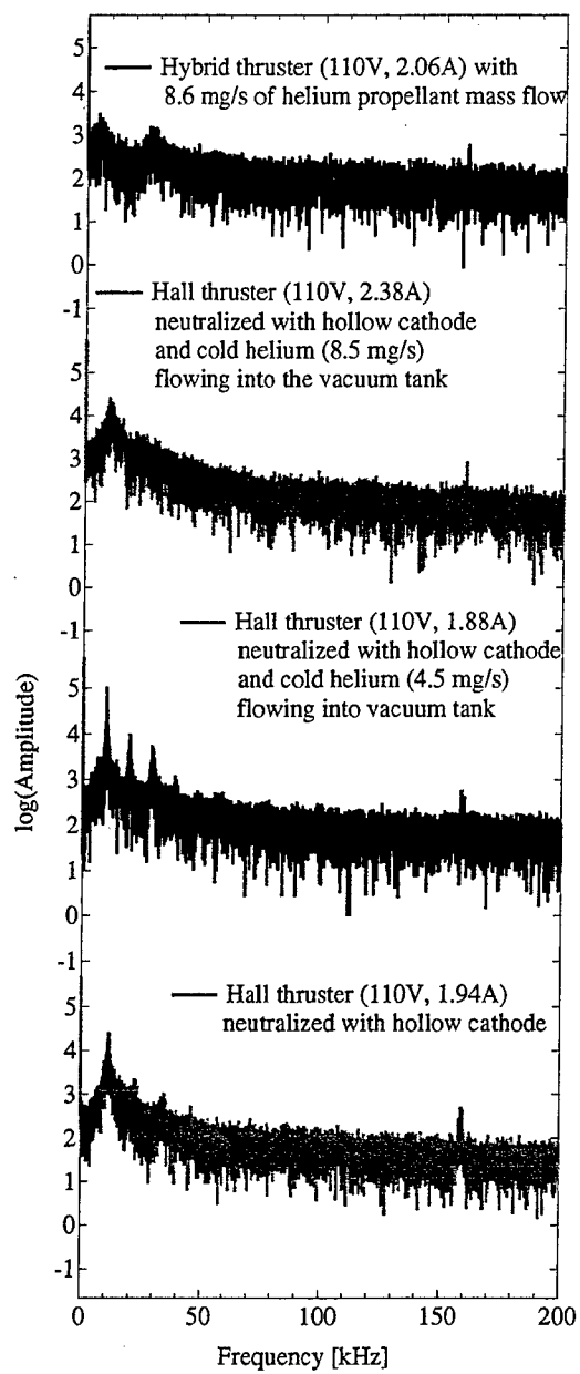
Figure 16. Comparison of Hall discharge current fluctuations with a Hall discharge voltage of 110V.
