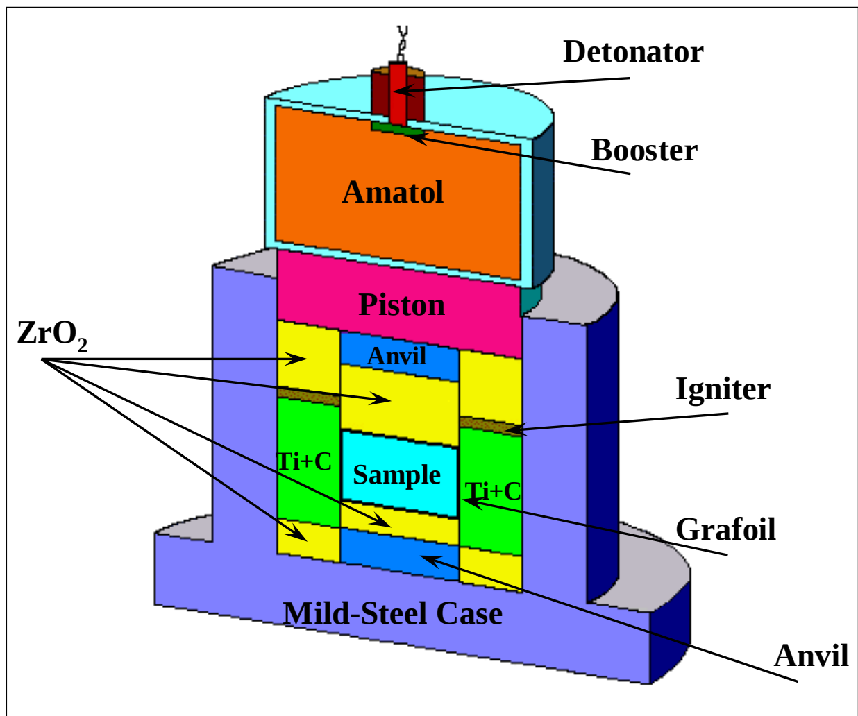
Figure 2. Schematic diagram of the HEC fixture.
