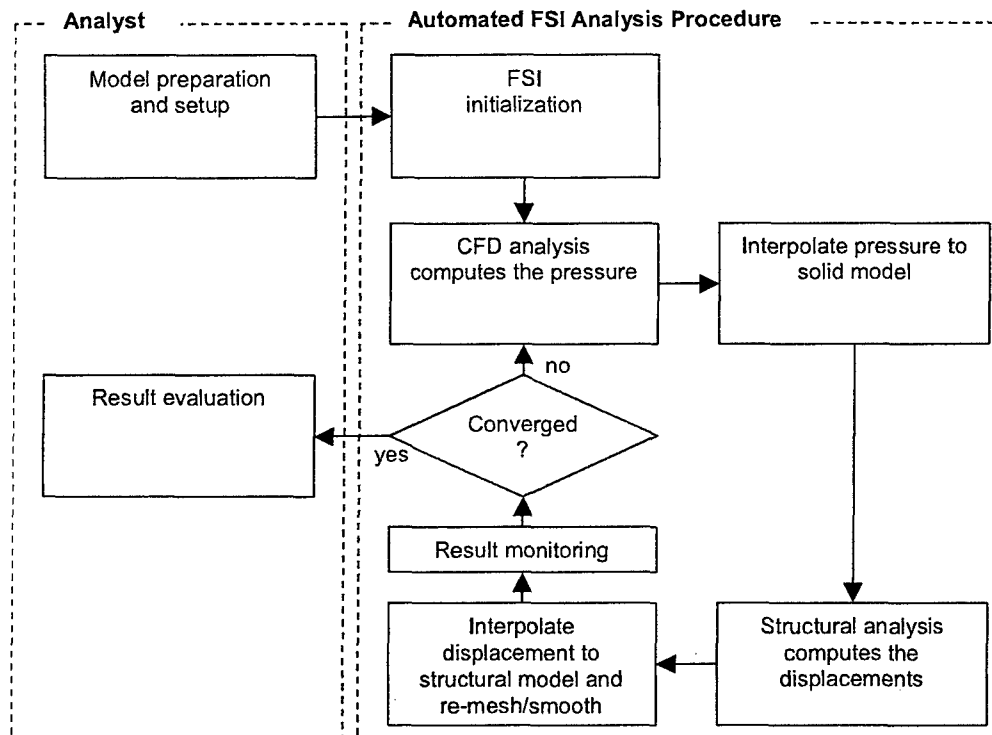
Figure 6: Basic Flowchart showing automated FSI analysis procedure
