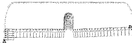
Figure 14: Pressure boundary conditions applied to element face group
