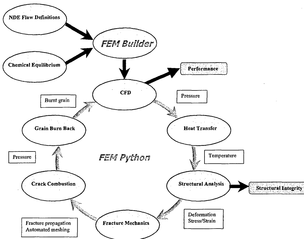
Figure 1: Possible FEM Builder solution sequence for solid rocket motors
