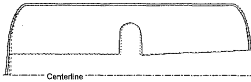
Figure 18: Solid model with E=500 psi showing initial and final propellant deformations
