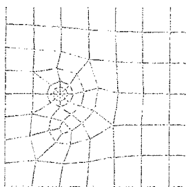
Figure 2 Crack insertion
