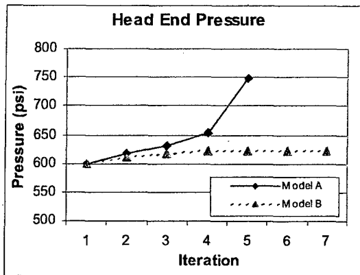
Figure 20: Plot of head end pressure for Model A and Model B
