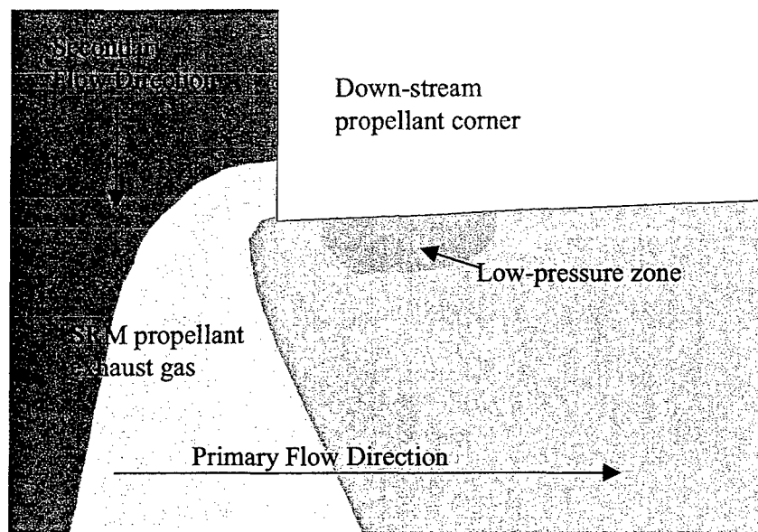
Figure 9: Pressure contours of 5.0 psi (34 kPa) of flow around a downstream corner of a segment joint/slot
