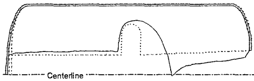
Figure 16: Solid model with E=200 psi showing initial and final propellant deformations
