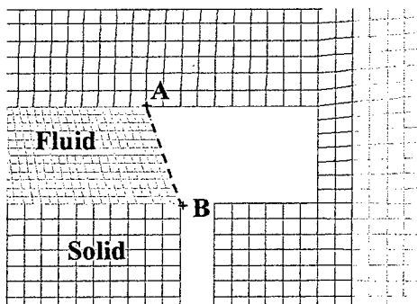
Figure 7: Pressure interpolation in a propellant joint/stress relief flap using a segmented line as an intermediate step
