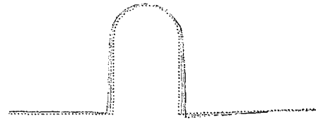
Figure 19: Detail of slot with E=500 psi showing intermediate propellant deformations
