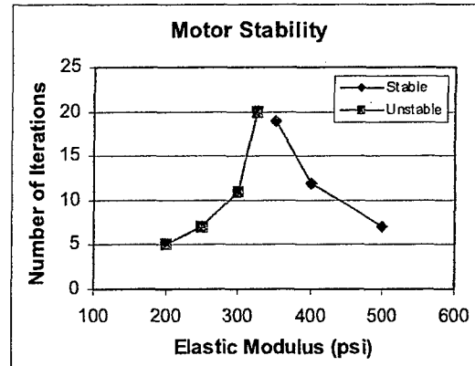
Figure 22: Plot of number of iterations vs. elastic modulus
