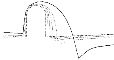
Figure 17: Detail of slot with E=200 psi showing intermediate propellant deformations
