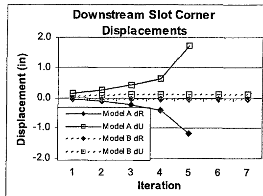
Figure 21: Plot of downstream slot corner displacement for Model A and Model B
