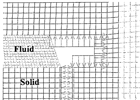
Figure 8: Pressure boundary conditions from pressure interpolation applied to structural model
