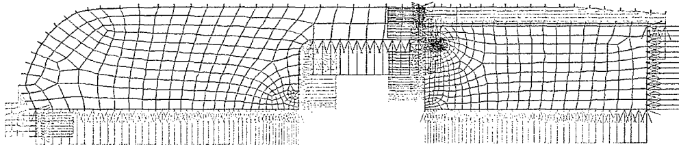
Figure 5 Interpolated pressure boundary condition colored by value
