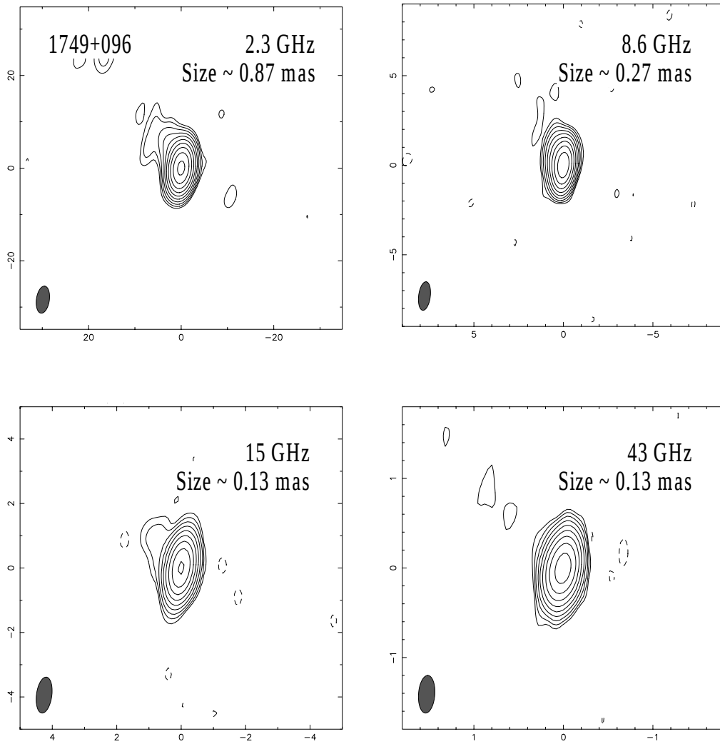
Figure 1. The radio frequency structure of the compact extragalactic source 1749+096 at four frequencies. The angular size (full width at half maximum) of a circular Gaussian component fitted to the data, together with the frequency of observation, is listed in each panel. Note the change in angular scale of the images from the lowest to the highest frequency.
