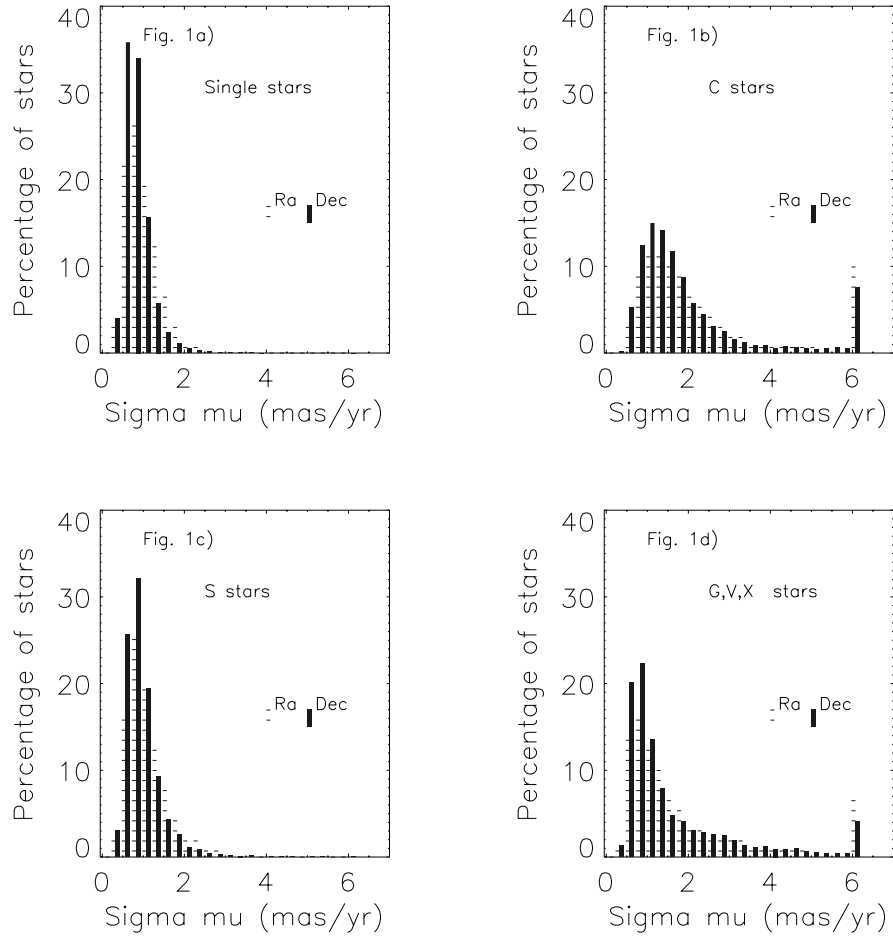
Figure 1. Percentage of stars by quoted Hipparcos standard error.
