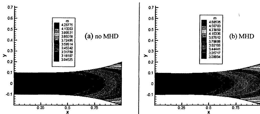
Figure 15 showing Mach number contours without and with MHD
