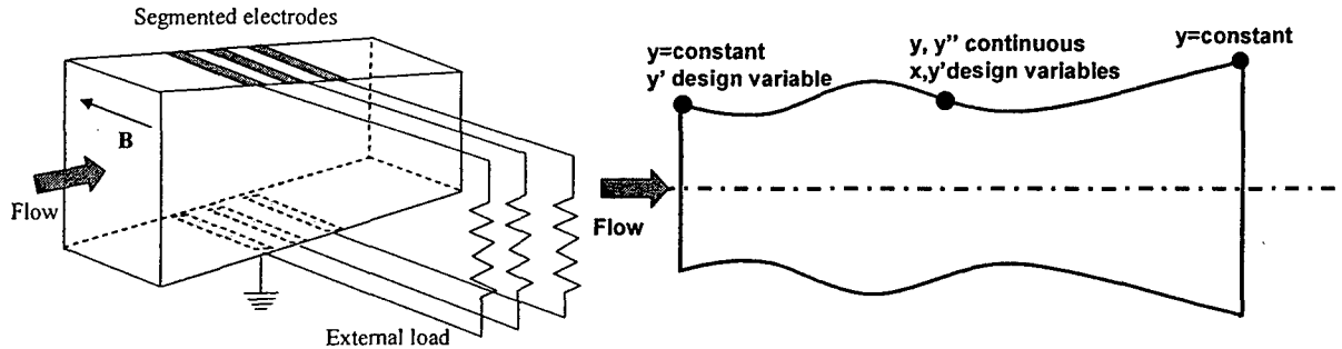
Figure 7: Schematic for MHD power generator optimization study
