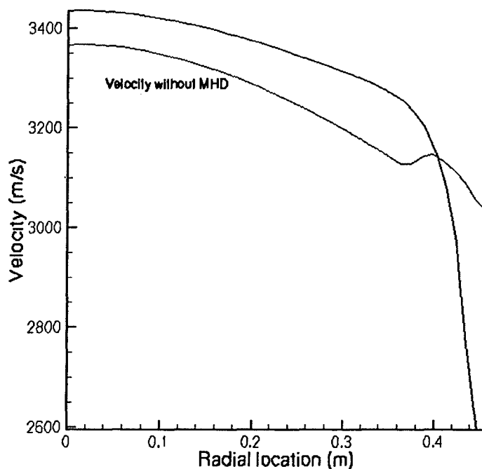
Figure 24: Exit plane velocity profile with and without MHD. Note the sharper drop in the velocity near the wall with MHD.
