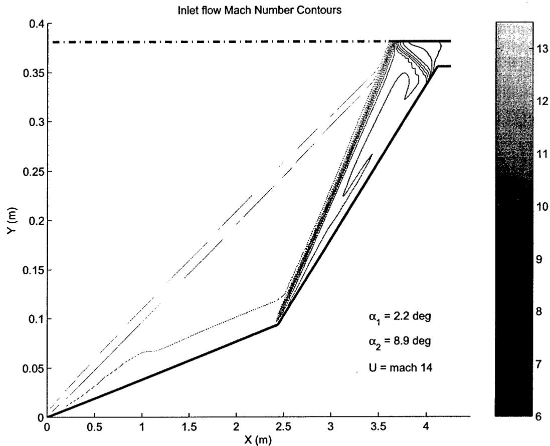
Figure 4.5 Mach contours of optimized cowl inlet.
