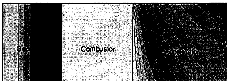
Figure 26: Contours of electric potential in the straight duct accelerator
