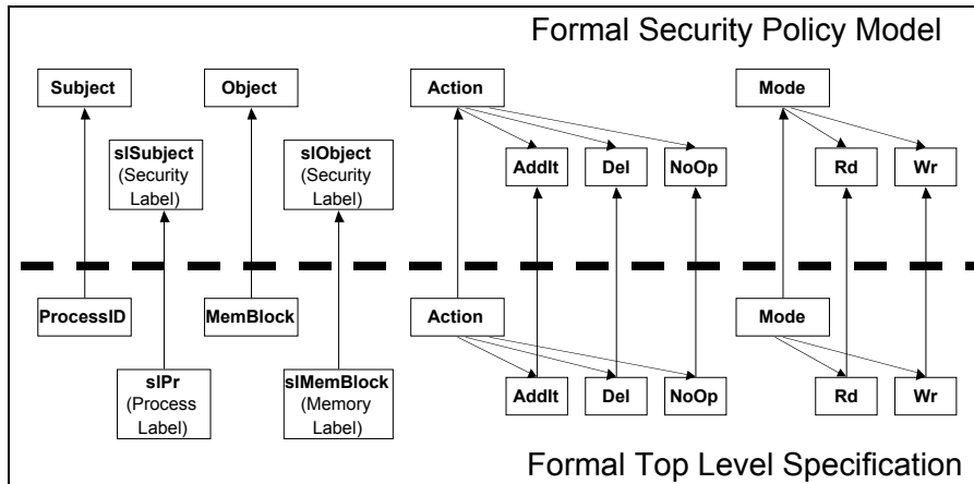
Figure 1: Intra-Level Mapping
